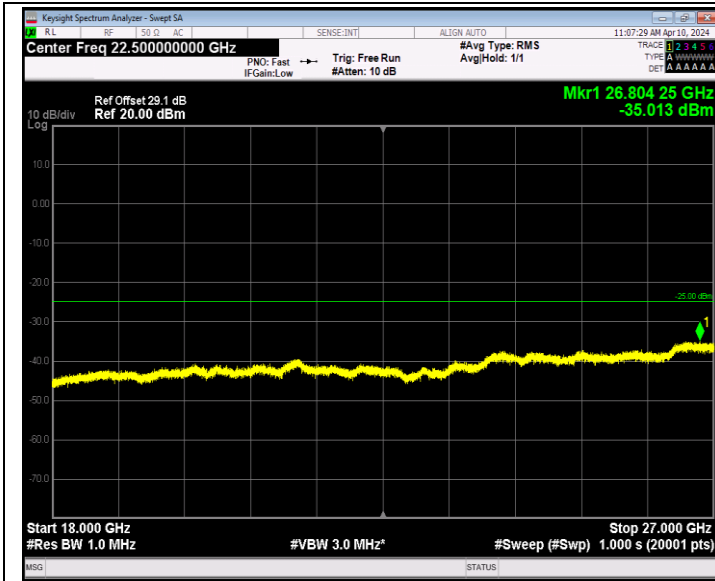
Band7_20MHz_QPSK_21100_1RB#0_18000~27000_18000~27000
