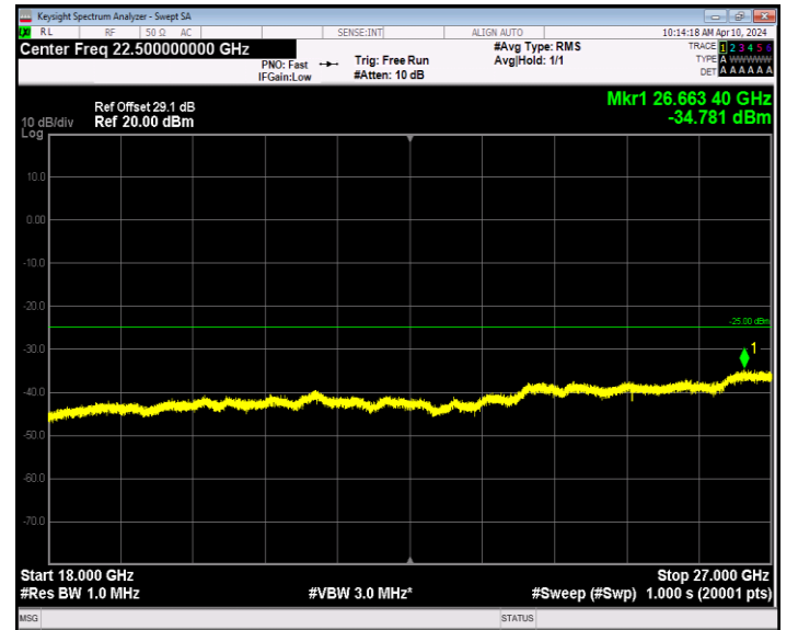
Band7_5MHz_16QAM_20775_1RB#0_18000~27000_18000~27000 00
