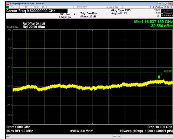
Band7_5MHz_16QAM_20775_1RB#0_1000~18000_1000~18000
