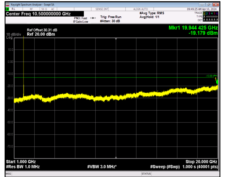
Band2_20MHz_64QAM_19100_1RB#0_1000~20000_1000~2000 0
