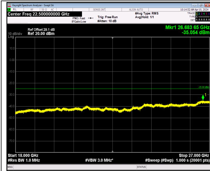
Band7_5MHz_64QAM_20775_1RB#0_18000~27000_18000~27000
