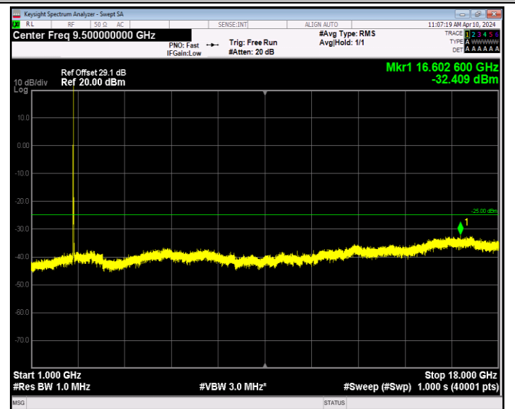
Band7_20MHz_QPSK_21100_1RB#0_1000~18000_1000~18000
