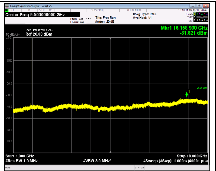
Band7_5MHz_64QAM_21425_1RB#0_1000~18000_1000~18000
