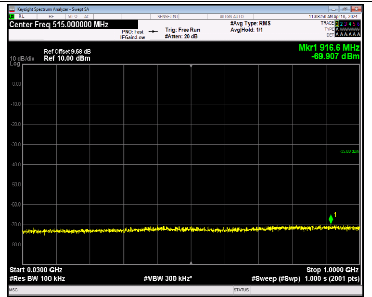
Band7_20MHz_QPSK_21350_1RB#0_30~1000_30~1000
