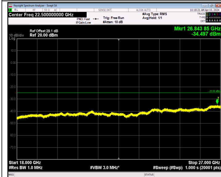
Band7_5MHz_64QAM_21425_1RB#0_18000~27000_18000~27000 00
