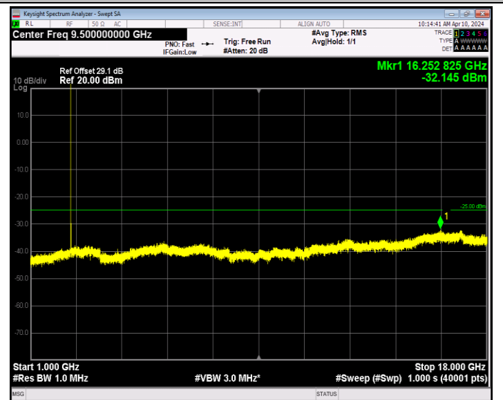
Band7_5MHz_64QAM_20775_1RB#0_1000~18000_1000~18000
