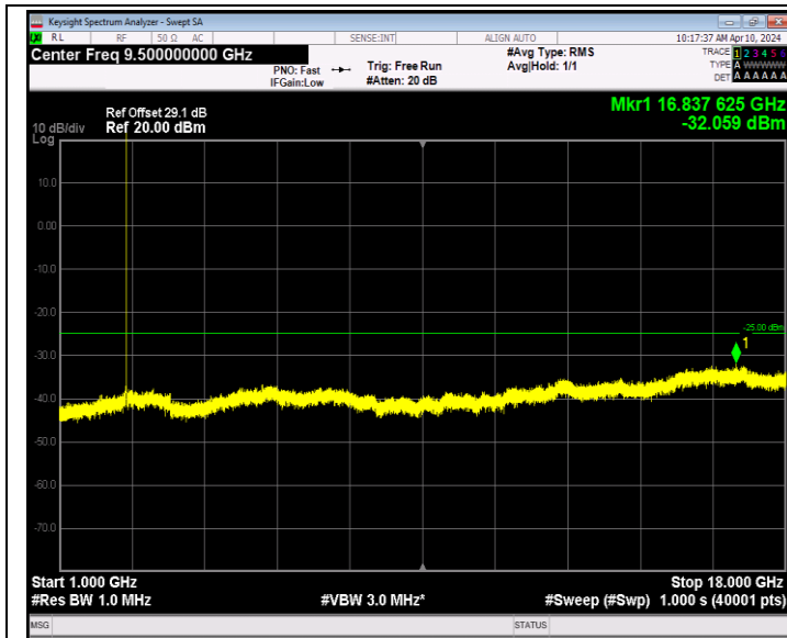
Band7_5MHz_16QAM_21425_1RB#0_1000~18000_1000~18000
