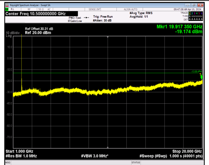
Band2_20MHz_64QAM_18700_1RB#0_1000~20000_1000~2000 0
