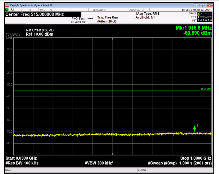
Band7_5MHz_64QAM_21100_1RB#0_30~1000_30~1000
