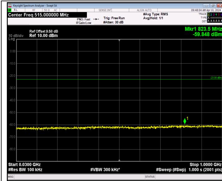
Band2_20MHz_64QAM_18900_1RB#0_30~1000_30~1000
