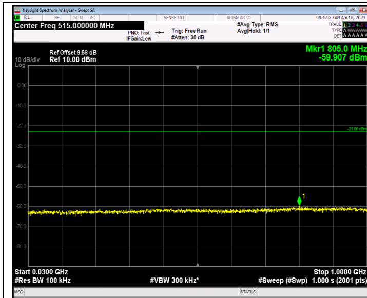
Band2_20MHz_QPSK_18900_1RB#0_30~1000_30~1000
