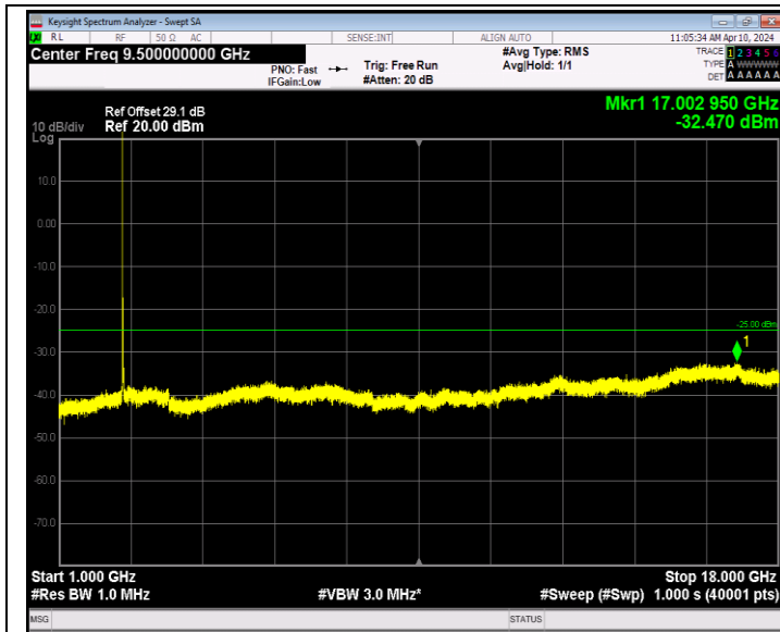
Band7_20MHz_QPSK_20850_1RB#0_1000~18000_1000~18000
