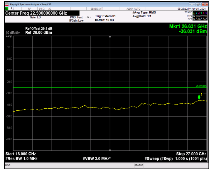
Band41_5MHz_QPSK_40620_1RB#0_18000~27000_18000~27000
