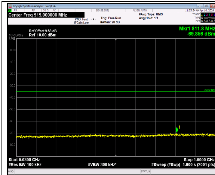
Band7_20MHz_16QAM_20850_1RB#0_30~1000_30~1000
