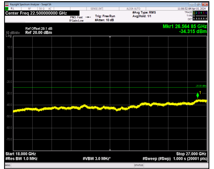
Band7_20MHz_64QAM_20850_1RB#0_18000~27000_18000~27000
