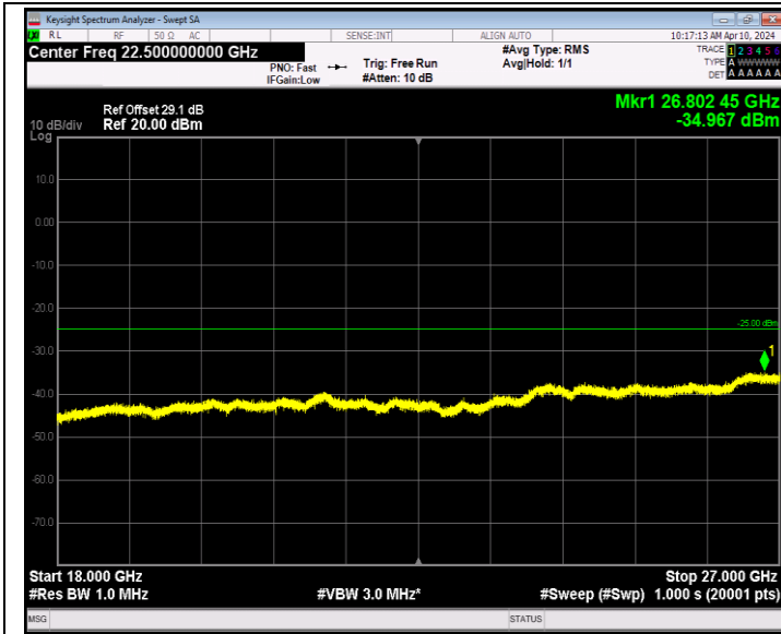
Band7_5MHz_QPSK_21425_1RB#0_18000~27000_18000~27000 0
