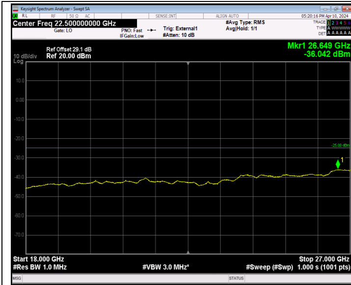
Band41_5MHz_QPSK_39675_1RB#0_18000~27000_18000~27000
