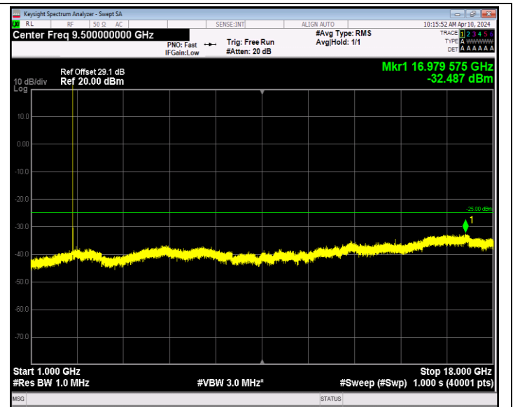
Band7_5MHz_16QAM_21100_1RB#0_1000~18000_1000~18000
