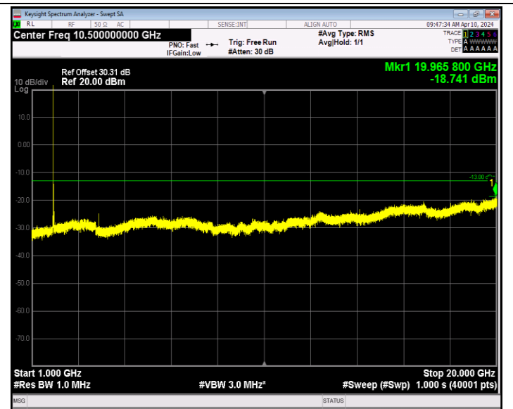
Band2_20MHz_QPSK_18900_1RB#0_1000~20000_1000~20000
