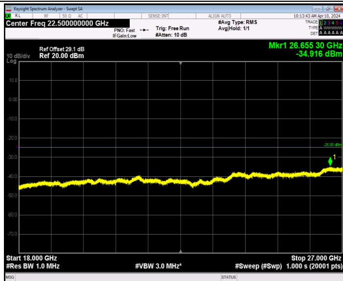
Band7_5MHz_QPSK_20775_1RB#0_18000~27000_18000~2700
