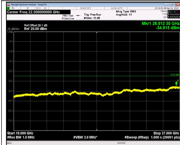
Band7_5MHz_16QAM_21100_1RB#0_18000~27000_18000~27000 00
