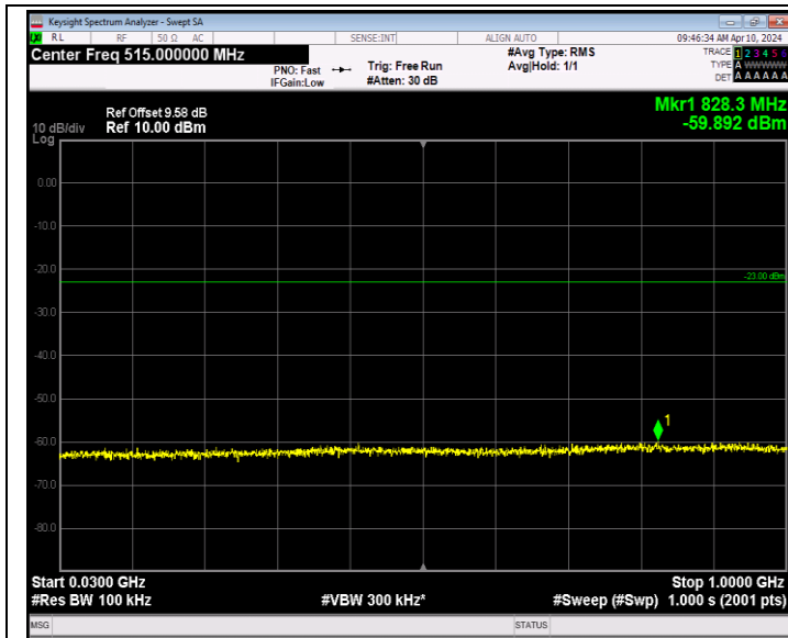
Band2_20MHz_16QAM_18700_1RB#0_30~1000_30~1000
