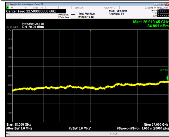
Band7_20MHz_16QAM_21350_1RB#0_18000~27000_18000~27000
