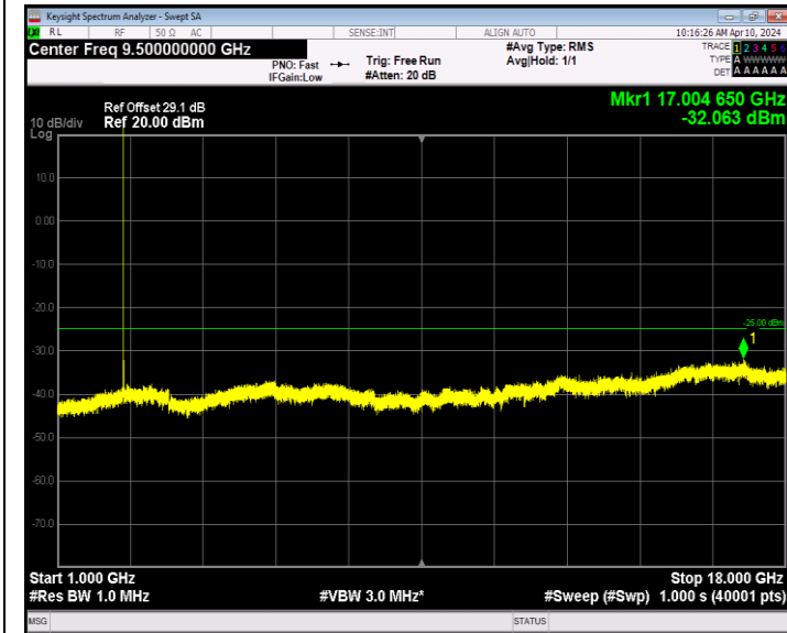
Band7_5MHz_64QAM_21100_1RB#0_1000~18000_1000~18000
