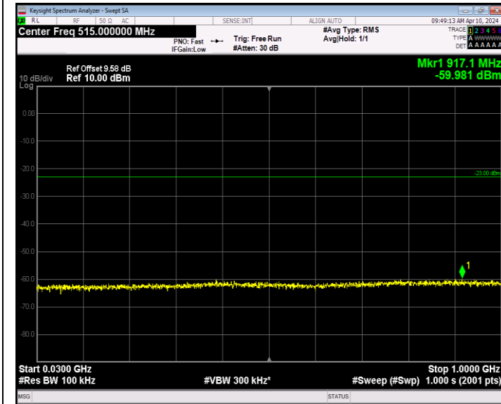
Band2_20MHz_64QAM_19100_1RB#0_30~1000_30~1000
