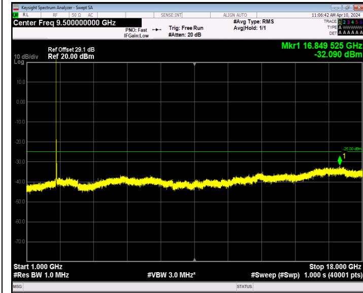
Band7_20MHz_64QAM_20850_1RB#0_1000~18000_1000~18000
