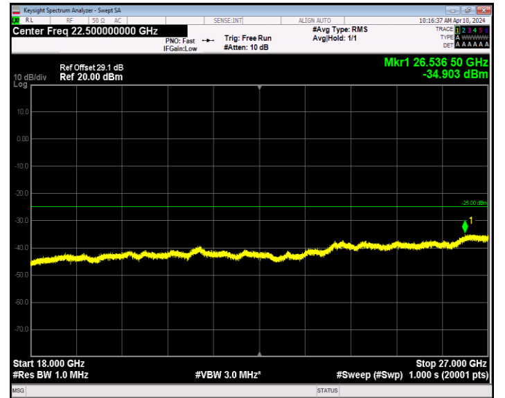
Band7_5MHz_64QAM_21100_1RB#0_18000~27000_18000~27000
