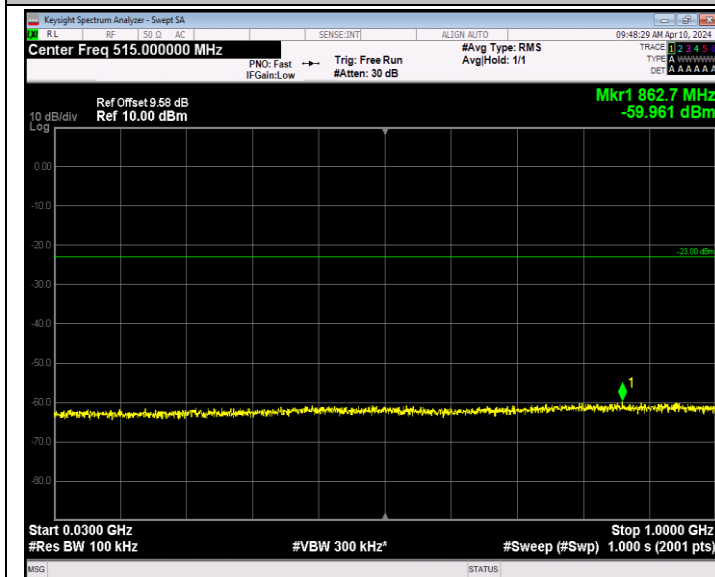
Band2_20MHz_QPSK_19100_1RB#0_30~1000_30~1000
