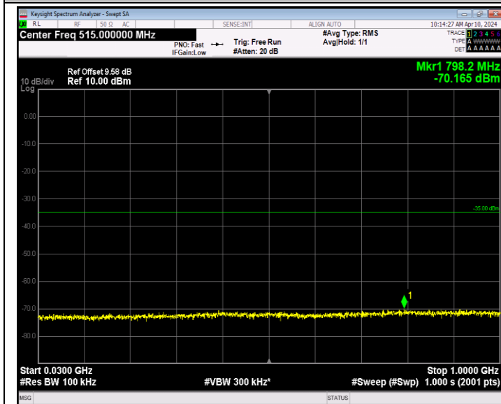
Band7_5MHz_64QAM_20775_1RB#0_30~1000_30~1000
