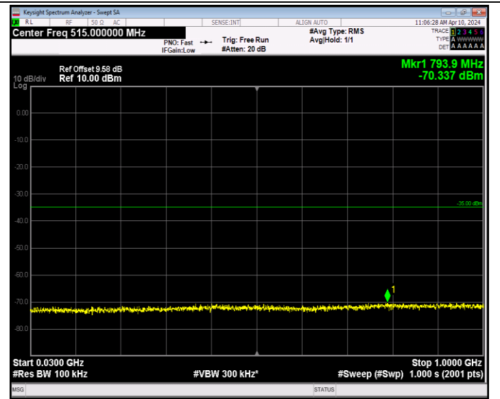
Band7_20MHz_64QAM_20850_1RB#0_30~1000_30~1000
