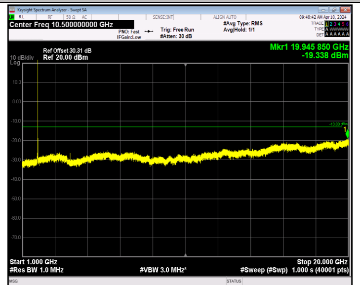
Band2_20MHz_QPSK_19100_1RB#0_1000~20000_1000~20000
