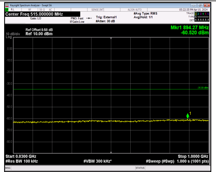
Band41_5MHz_QPSK_40620_1RB#0_30~1000_30~1000
