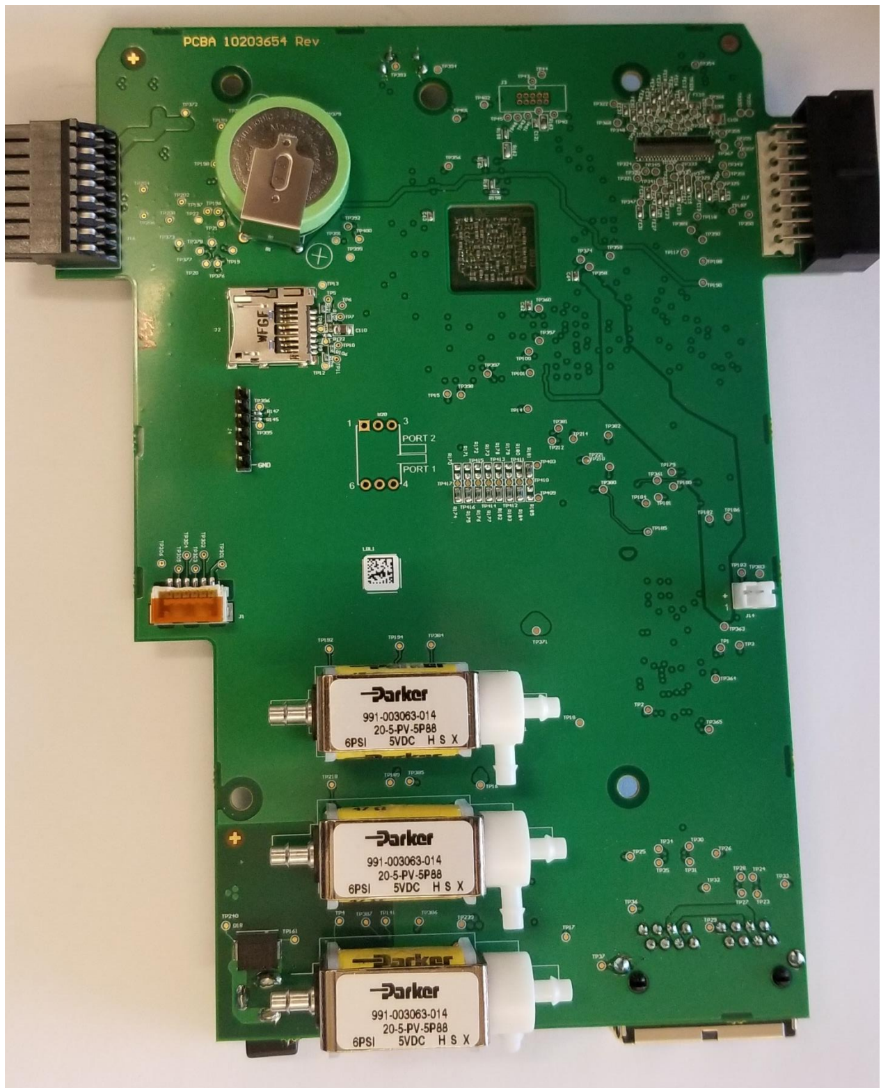
Figure 4 - Test Stand Bottom
