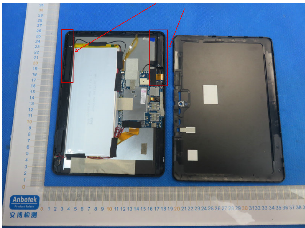
2G & 3G and 4G Antenna
