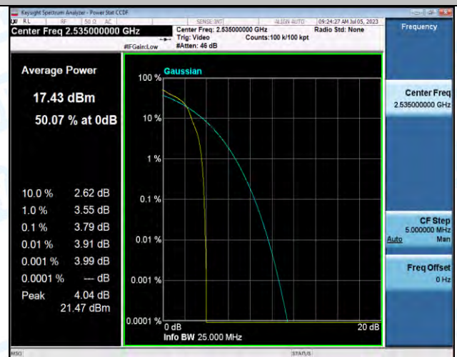
Band7-10MHz-16QAM-21100-1RB#0-PASS
