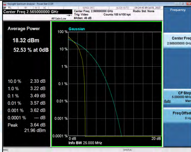
Band7-10MHz-QPSK-21400-1RB#0-PASS
