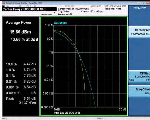
Band41-20MHz-QPSK-41490-100RB#0-PASS
