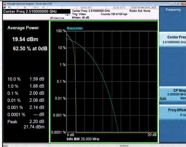
Band7-20MHz-QPSK-20850-1RB#0-PASS
