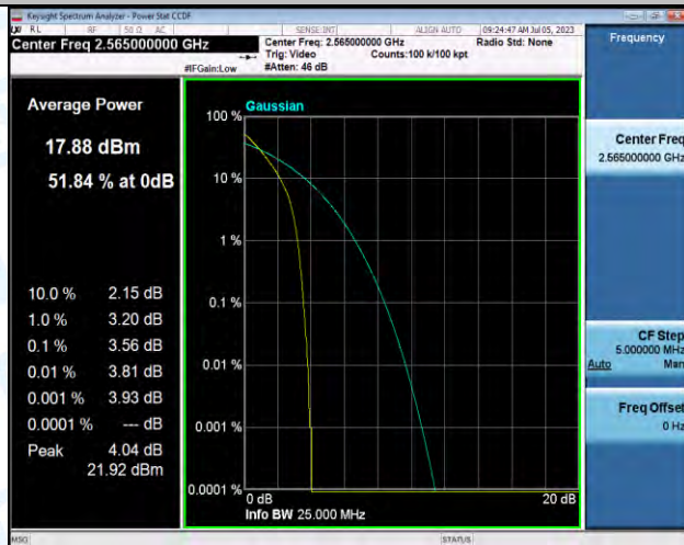
Band7-10MHz-QPSK-21400-50RB#0-PASS
