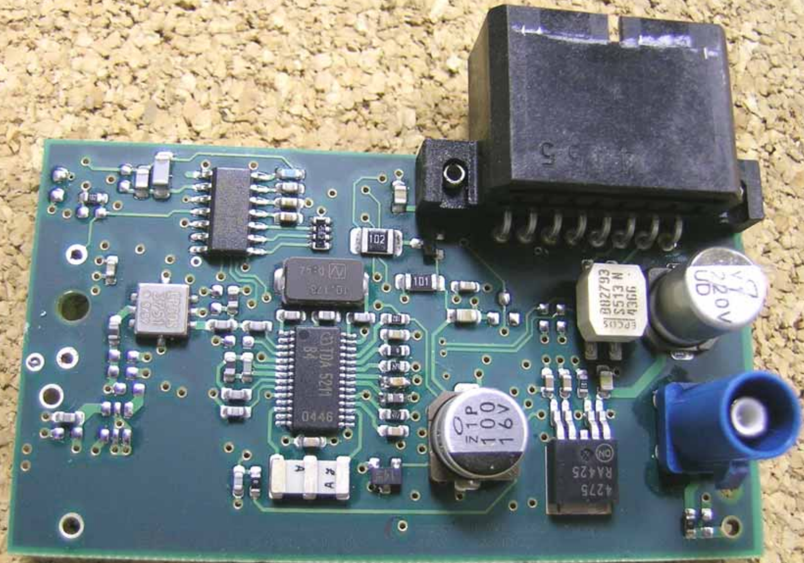
PCB (top)
