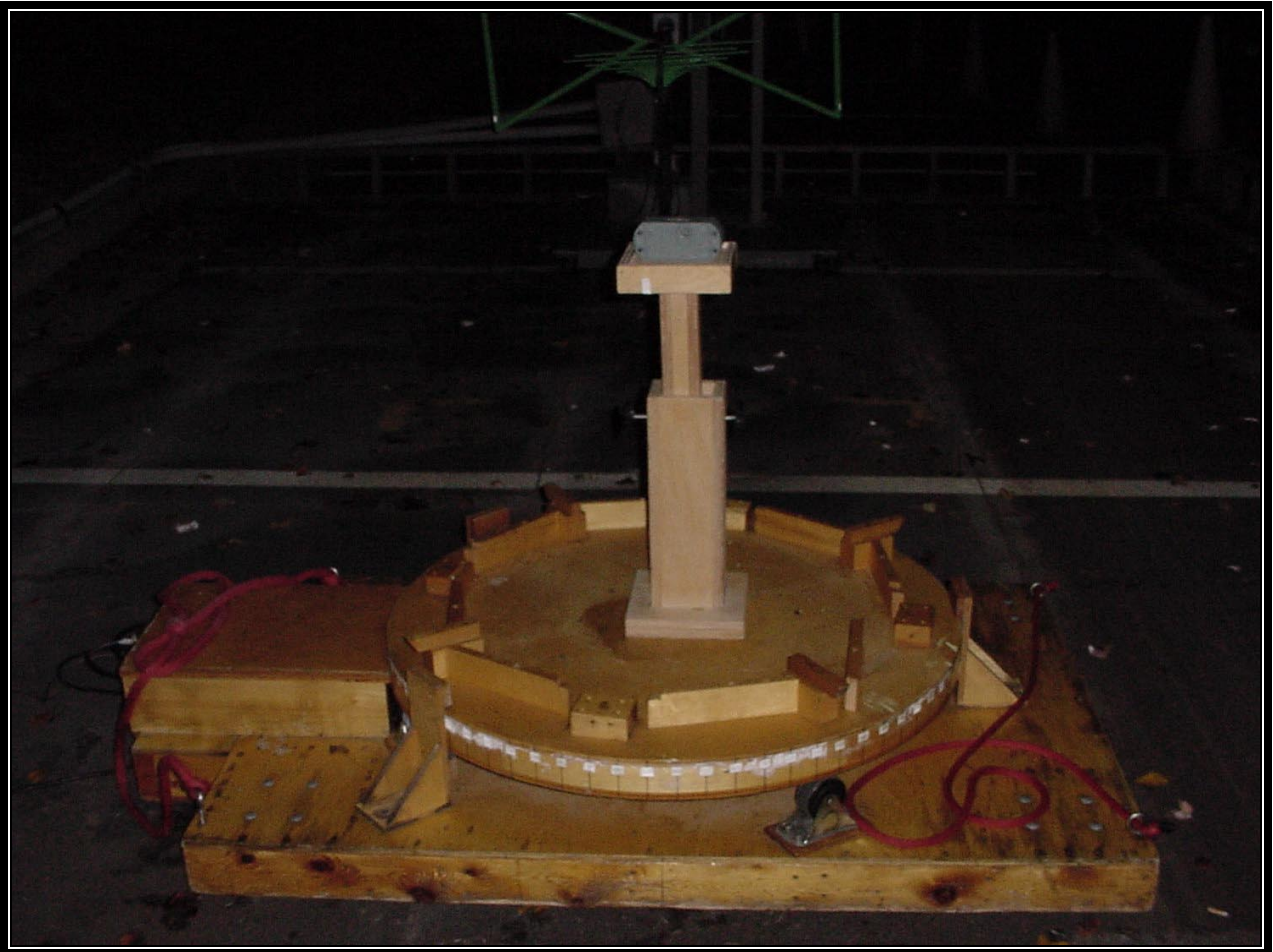
PHOTOGRAPH 3: RADIATED EMISSION REAR VIEW, WORST CASE CONFIGURATION
