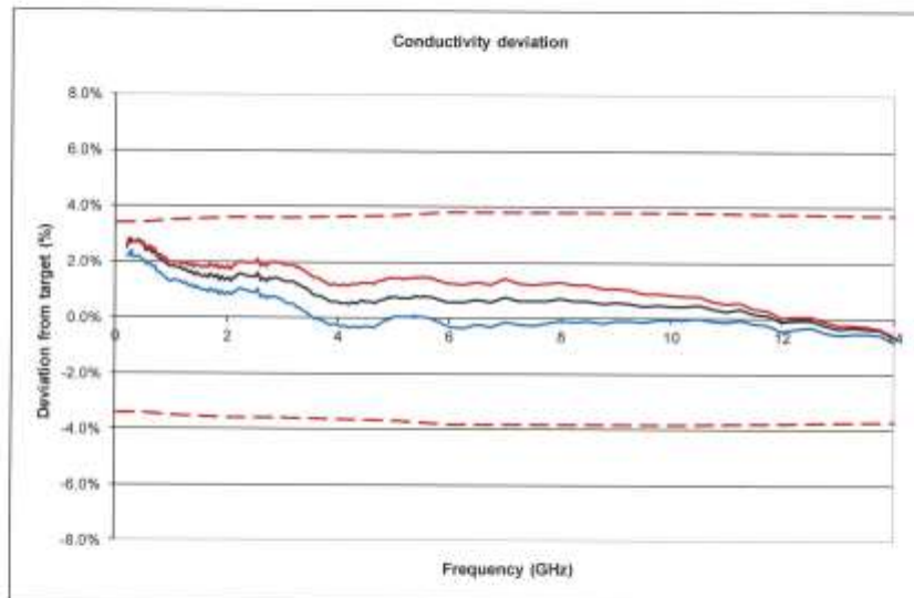
Fig. 4.2 HSL conductivity deviation from target, 200 MHz – 14 GHz
