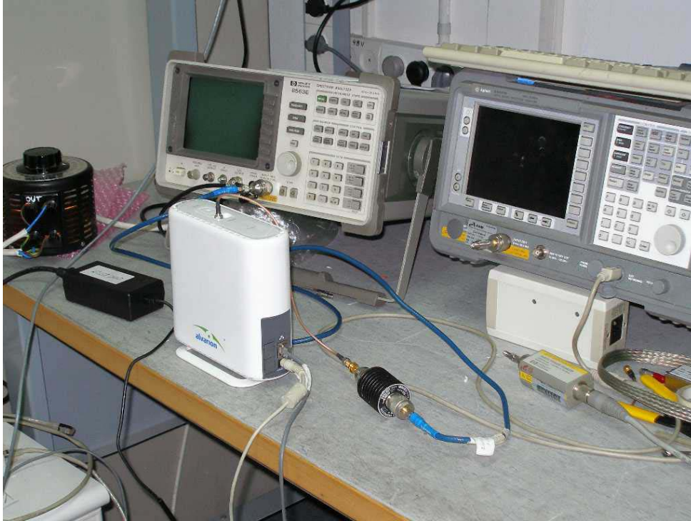
Test setup . BMAX-CPE- Si- E- 2.3
