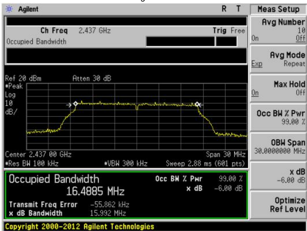
802.11g CH2437MHZ
