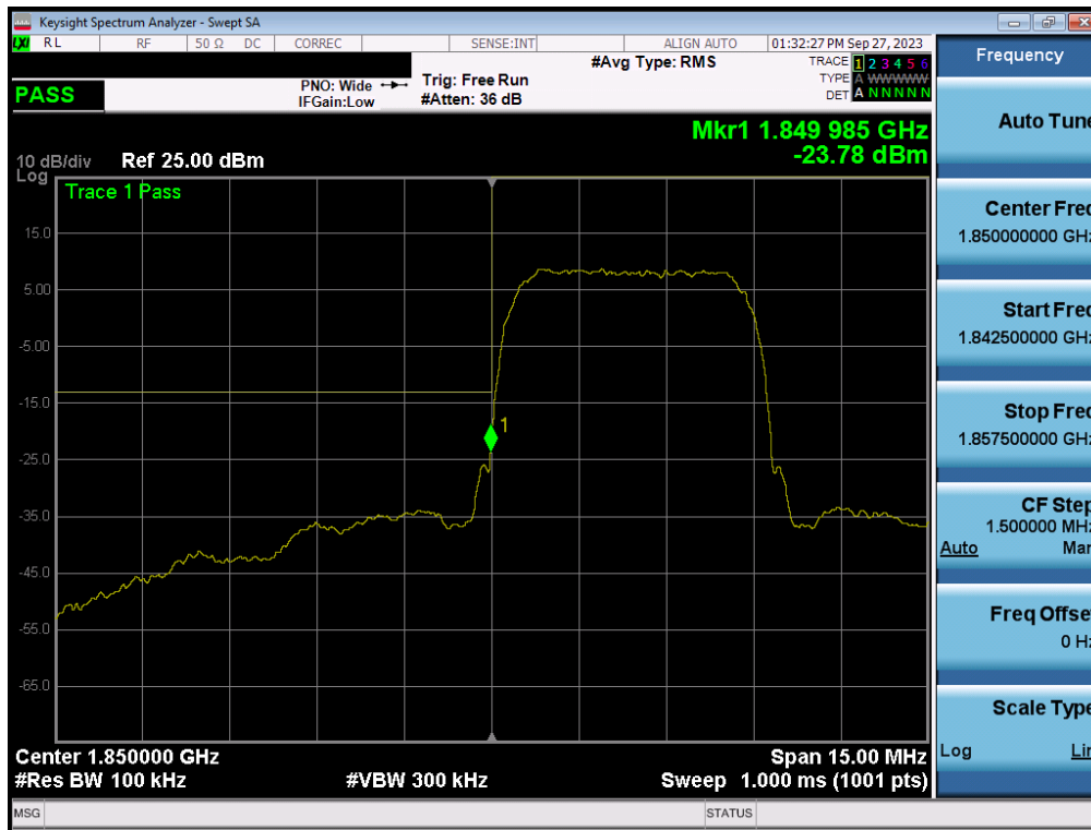
Plot 7-50. Lower Band Edge Plot (WCDMA PCS – Ch. 9262 - Ant1)
