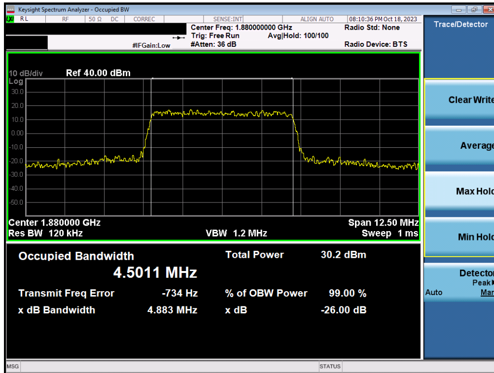
Plot 7-19. Occupied Bandwidth Plot (LTE Band 2 - 5MHz QPSK - Full RB - Ant2)
