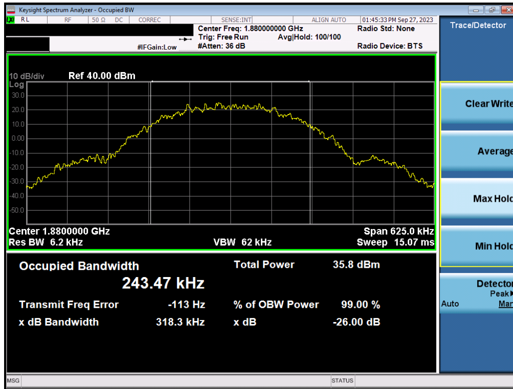
Plot 7-25. Occupied Bandwidth Plot (GPRS, Ch. 661 - Ant1)
