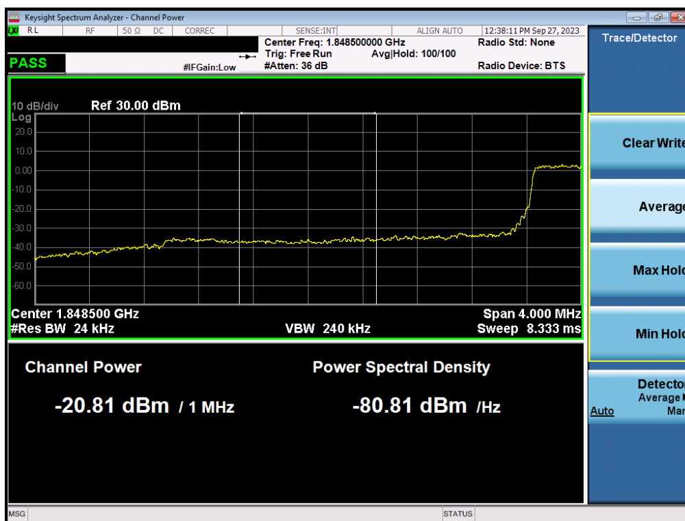
Plot 7-41. Extended Lower Band Edge Plot (LTE Band 2 - 3MHz QPSK – Full RB - Ant1)
