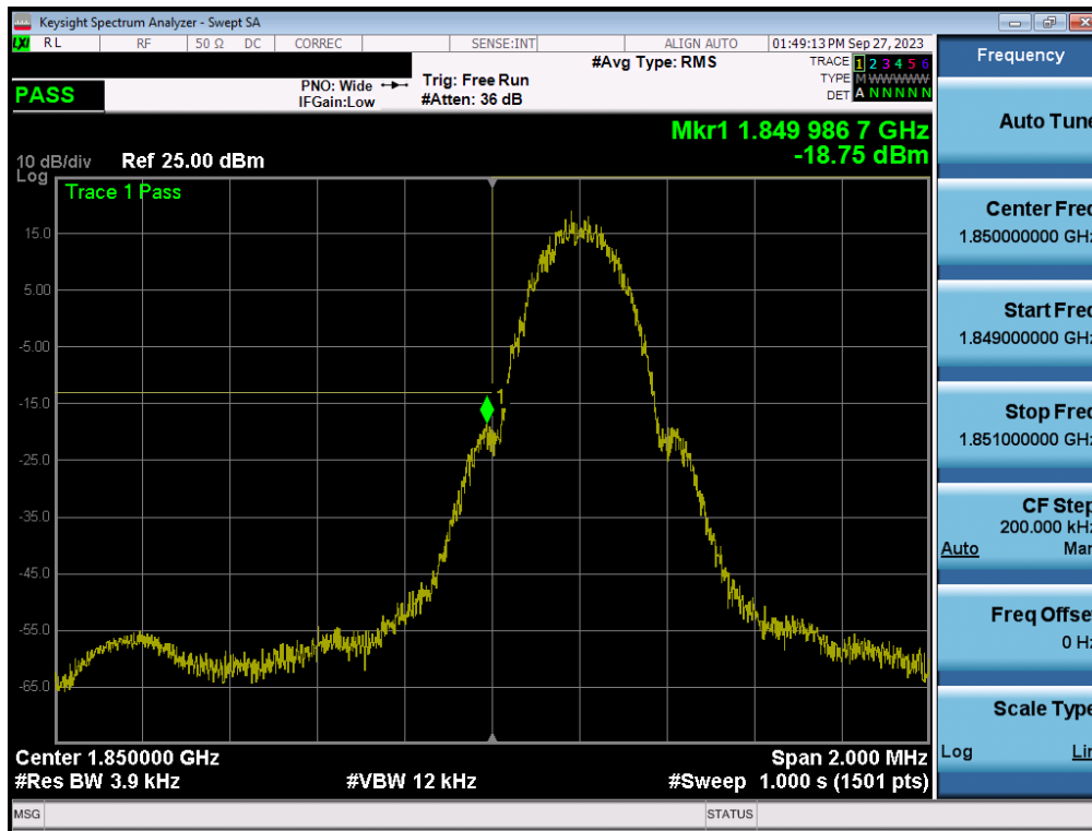
Plot 7-48. Lower Band Edge Plot (GPRS PCS – Ch. 512 - Ant1)
