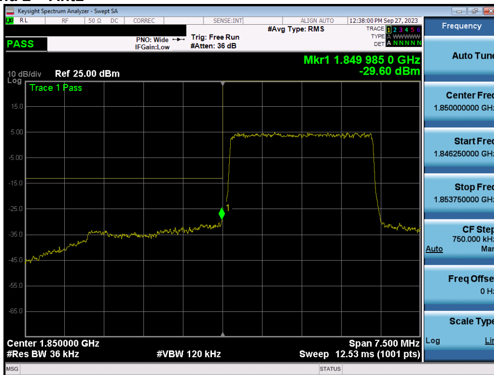
Plot 7-40. Lower Band Edge Plot (LTE Band 2 - 3MHz QPSK – Full RB - Ant1)
