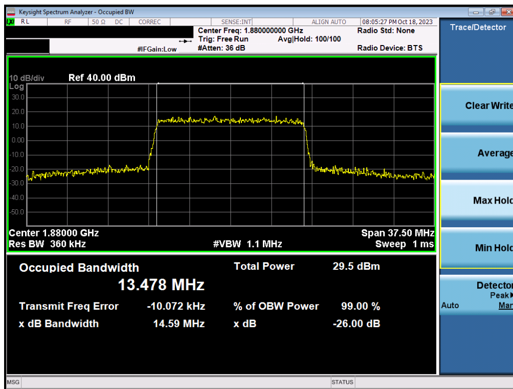
Plot 7-16. Occupied Bandwidth Plot (LTE Band 2 - 15MHz 16-QAM - Full RB - Ant2)
