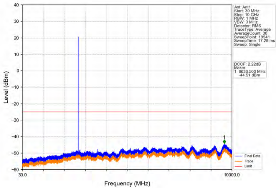
Band41_5MHz_64QAM_HCH_2687.5MHz_RB_1_0_NTN
