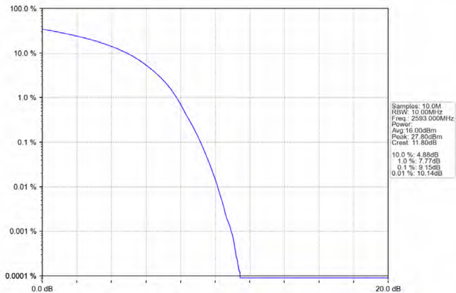
Band41_20MHz_64QAM_MCH_2593MHz_RB_100_0 NTN
