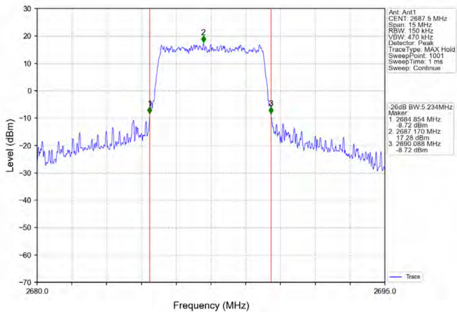
Band41_5MHz_16QAM_HCH_2687.5MHz_RB_25_0_NTV
