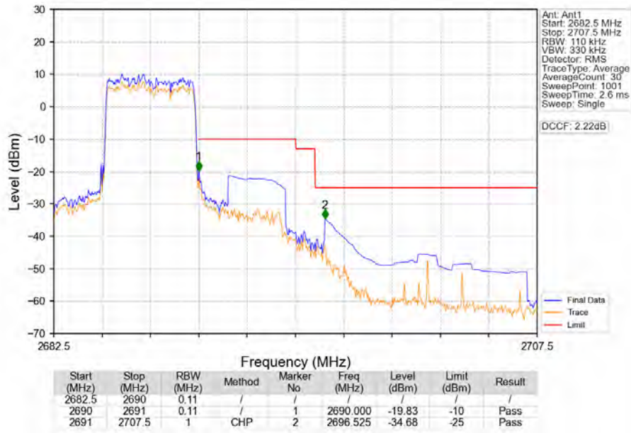
Band41 5MHz QPSK HCH 2687.5MHz RB 25 0 NTN
