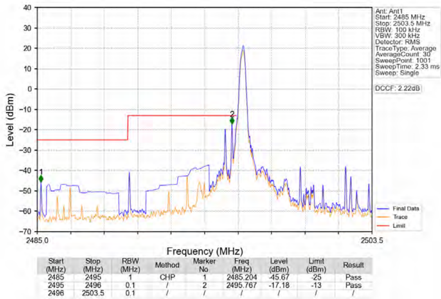
Band41 5MHz 64QAM LCH 2498.5MHz RB 1 0 NTNV
