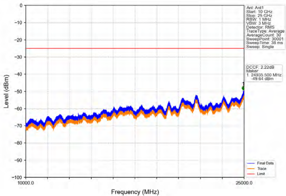
Band41_5MHz_64QAM_HCH_2687.5MHz_RB_1_0_NTN
