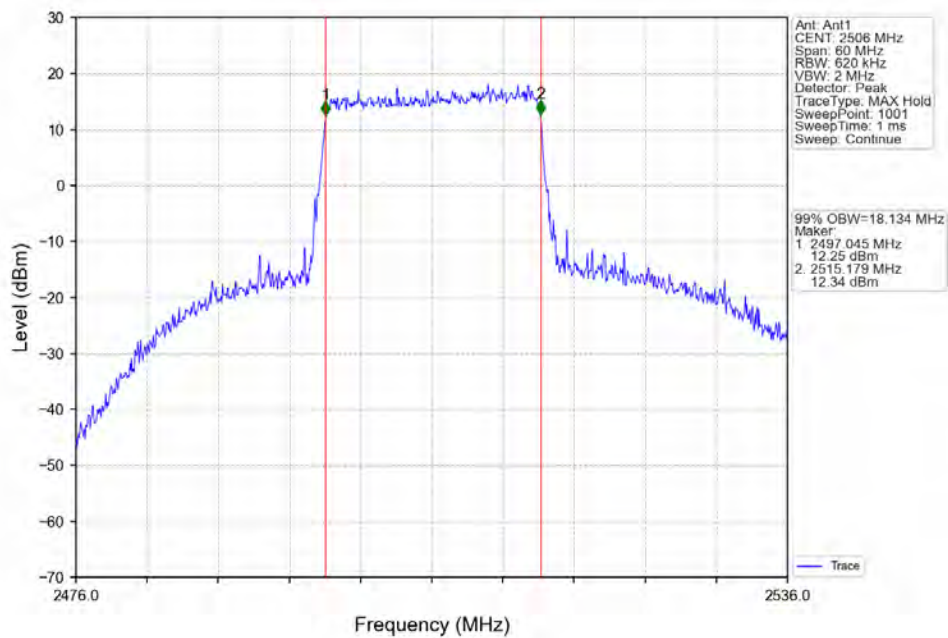
Band41_20MHz_64QAM_LCH_2506MHz_RB_100_0_NTN
