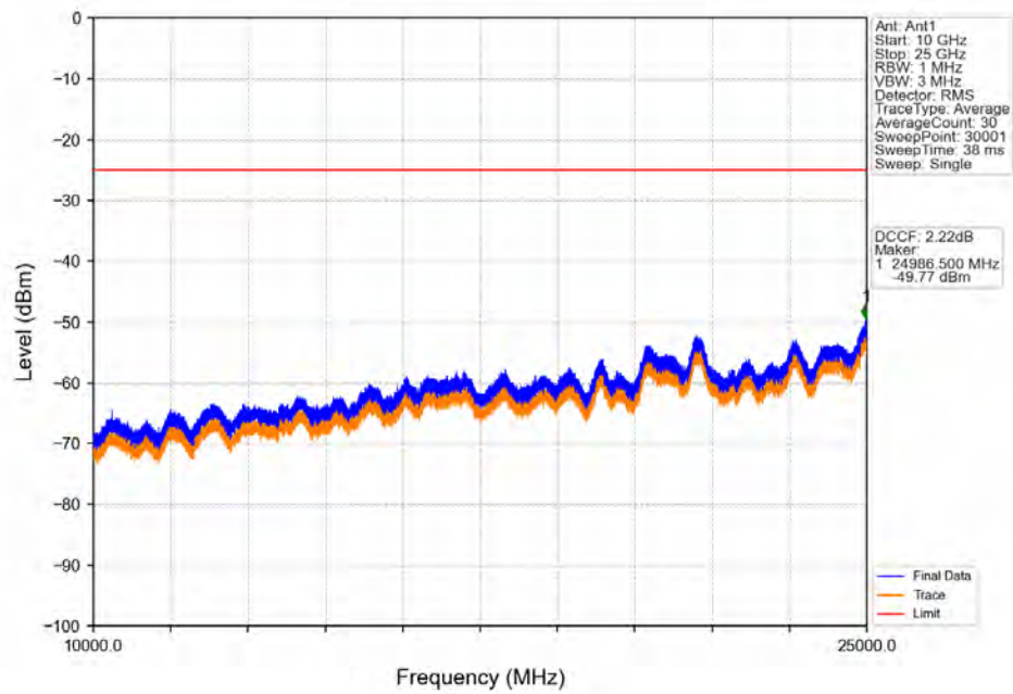
Band41_5MHz_64QAM_MCH_2593MHz_RB_1_0_NTNV
