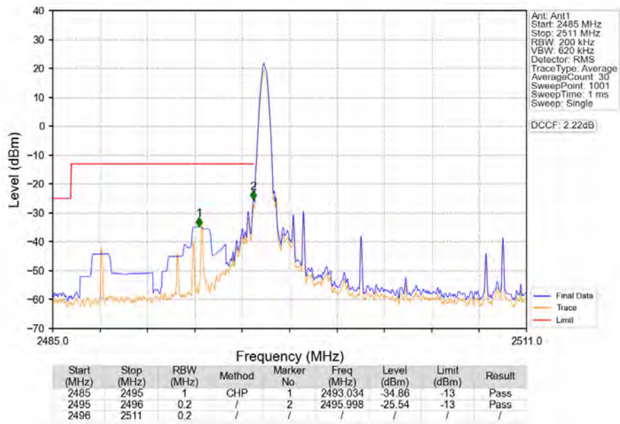
Band41_10MHz_64QAM_LCH_2501MHz_RB_1_0_NTNV
