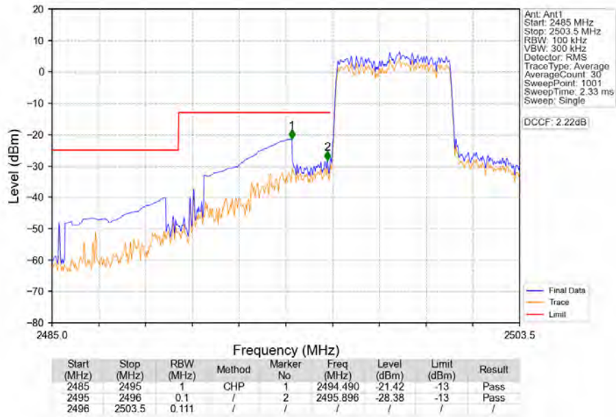
Band41 5MHz 64QAM LCH 2498.5MHz RB 25 0 NTNV
