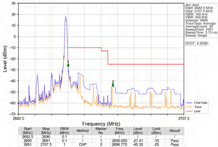
Band41_5MHz_64QAM_HCH_2687.5MHz_RB_1_24_NTN
