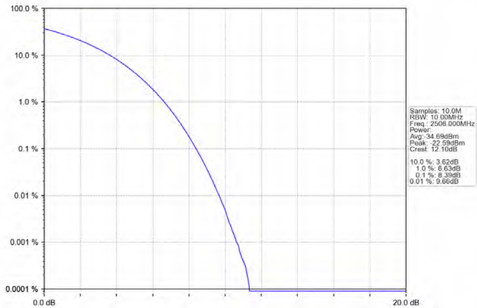
Band41 20MHz 64QAM LCH 2506MHz RB 100 0 NTN
