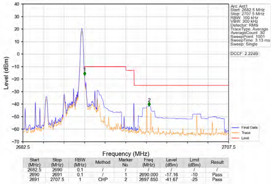
Band41 5MHz 16QAM HCH 2687.5MHz RB 1 24 NTN
