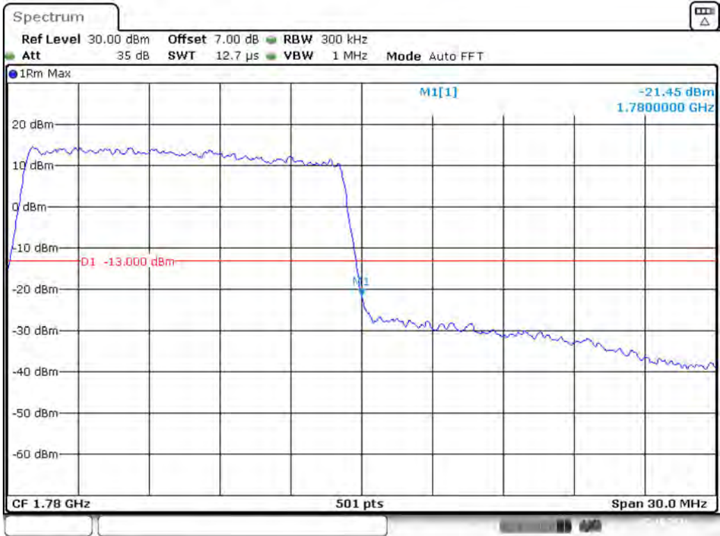
Band 66_15 MHz_High_QPSK_RB75#0
