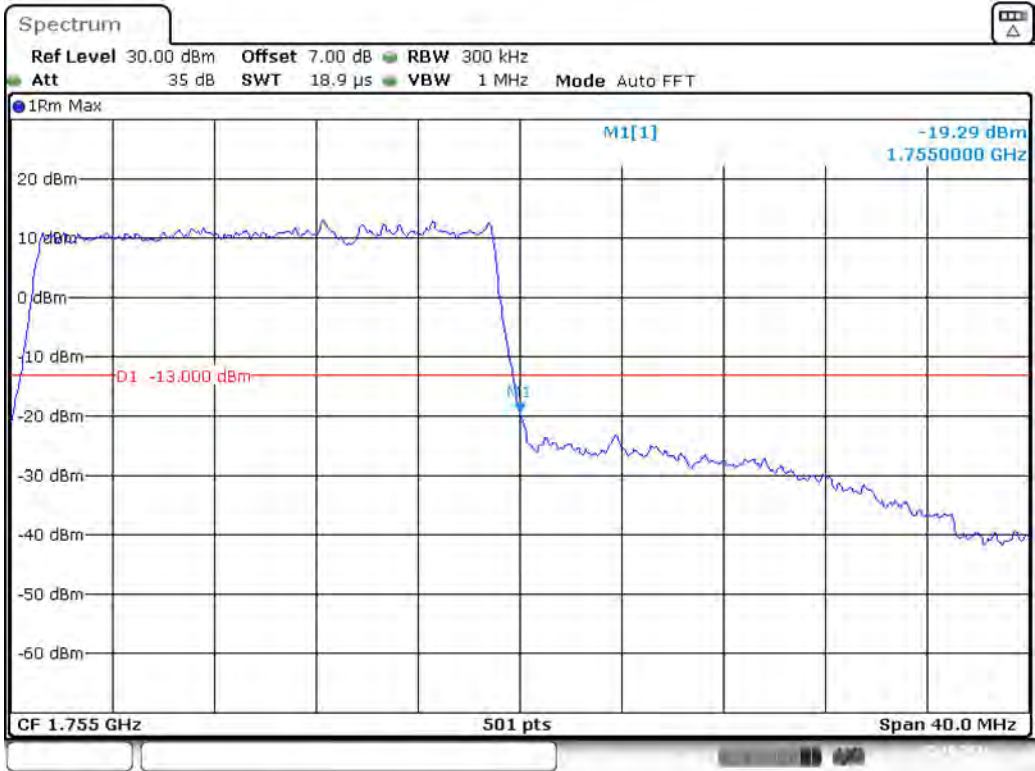
Band 4_20 MHz_High_QPSK_RB100#0
