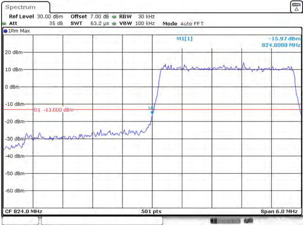
Band 5_3 MHz_Low_QPSK_RB15#0
