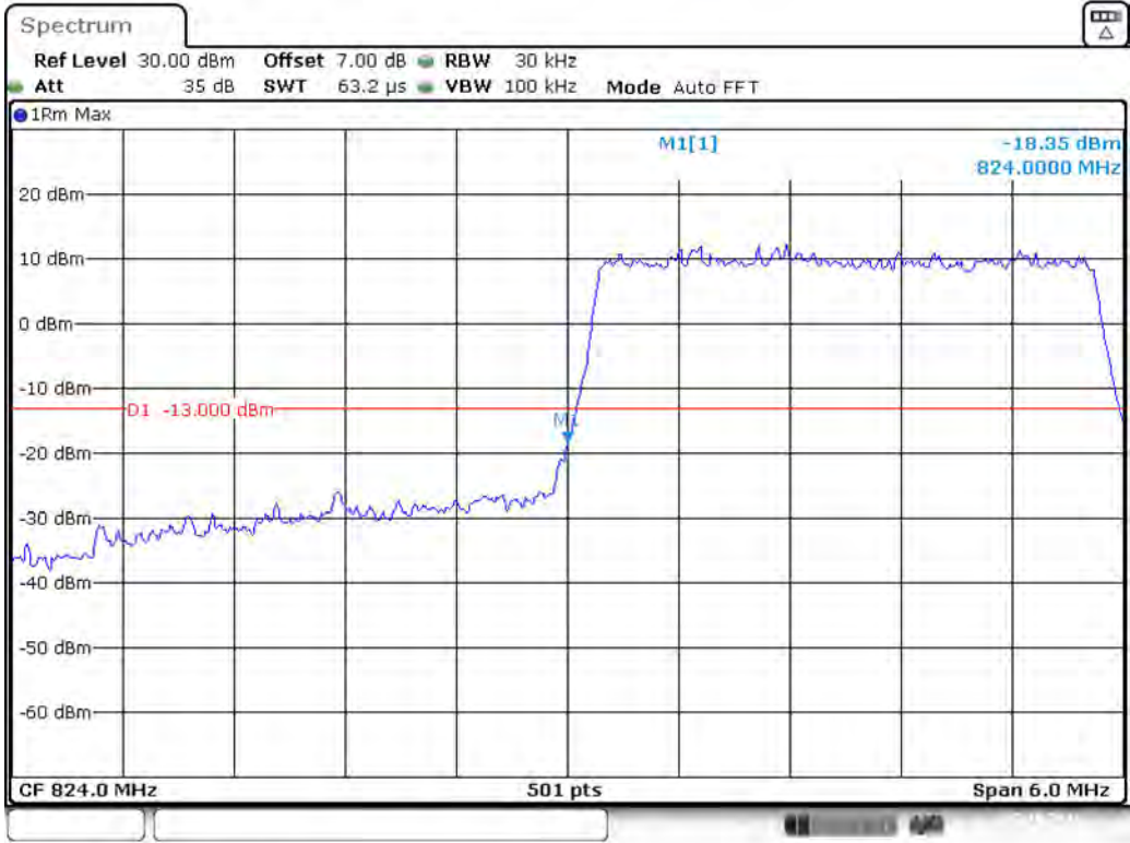
Band 5_3 MHz_Low_16QAM_RB15#0
