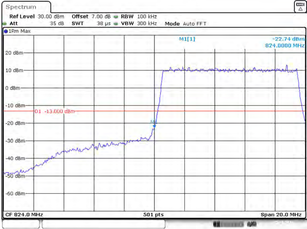
Band 5_10 MHz_Low_16QAM_RB50#0
