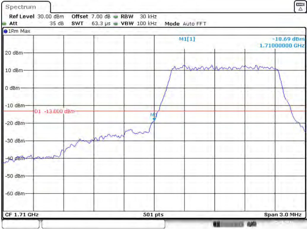
Band 4_1.4 MHz_Low_16QAM_RB6#0
