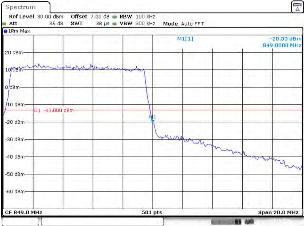
Band 5_10 MHz_High_QPSK_RB50#0
