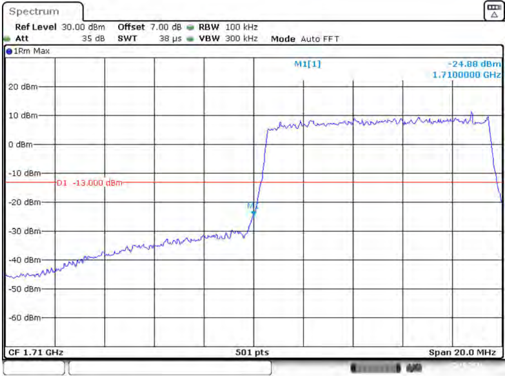
Band 4_10 MHz_Low_16QAM_RB50#0
