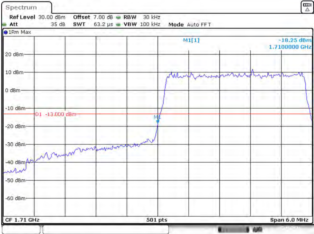
Band 4_3 MHz_Low_QPSK_RB15#0
