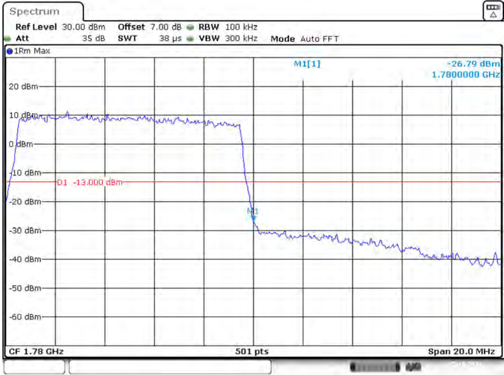
Band 66_10 MHz_High_16QAM_RB50#0
