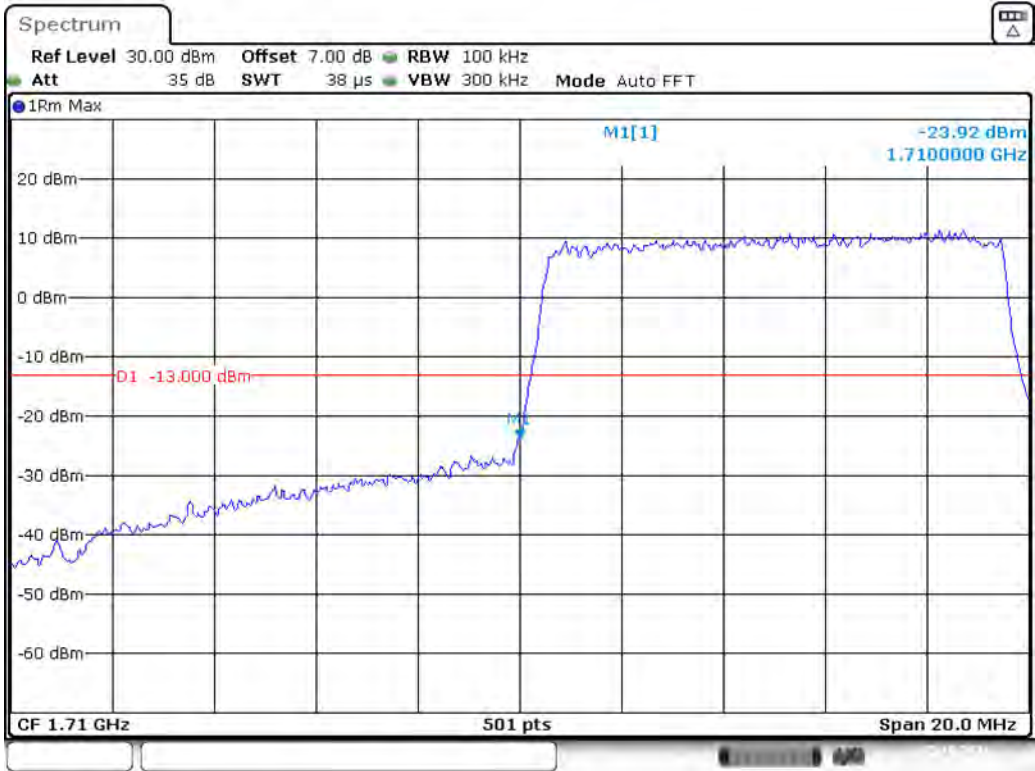
Band 66_10 MHz_Low_QPSK_RB50#0
