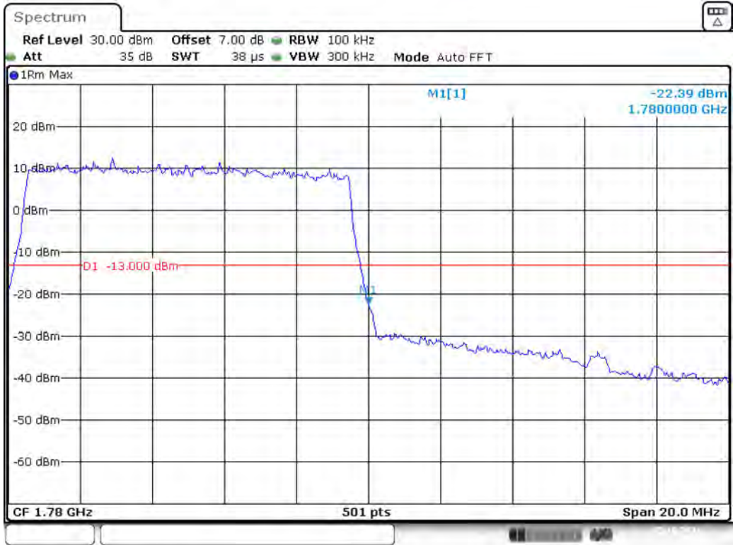
Band 66_10 MHz_High_QPSK_RB50#0
