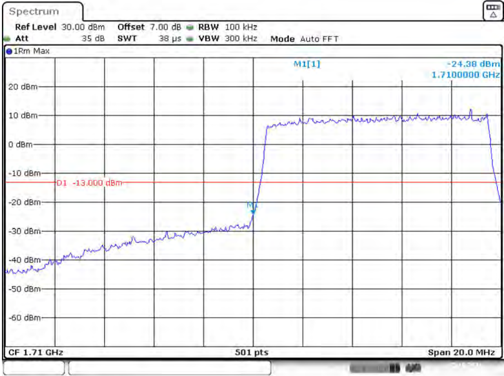
Band 66_10 MHz_Low_16QAM_RB50#0
