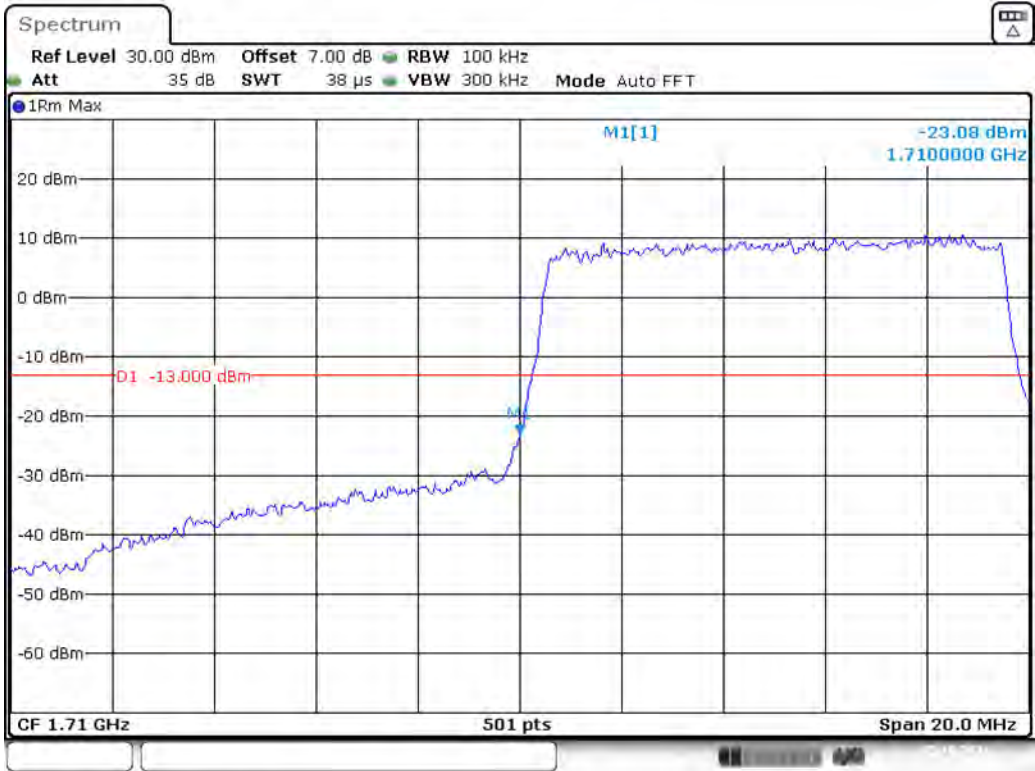
Band 4_10 MHz_Low_QPSK_RB50#0
