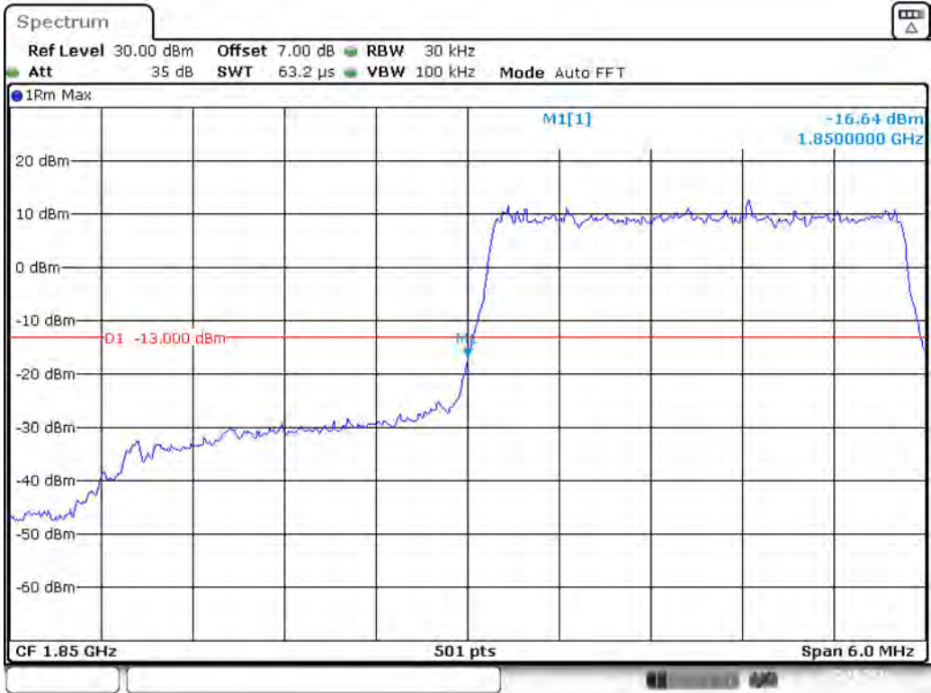
Band 2_3 MHz_Low_QPSK_RB15#0
