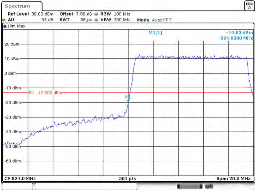
Band 5_10 MHz_Low_QPSK_RB50#0
