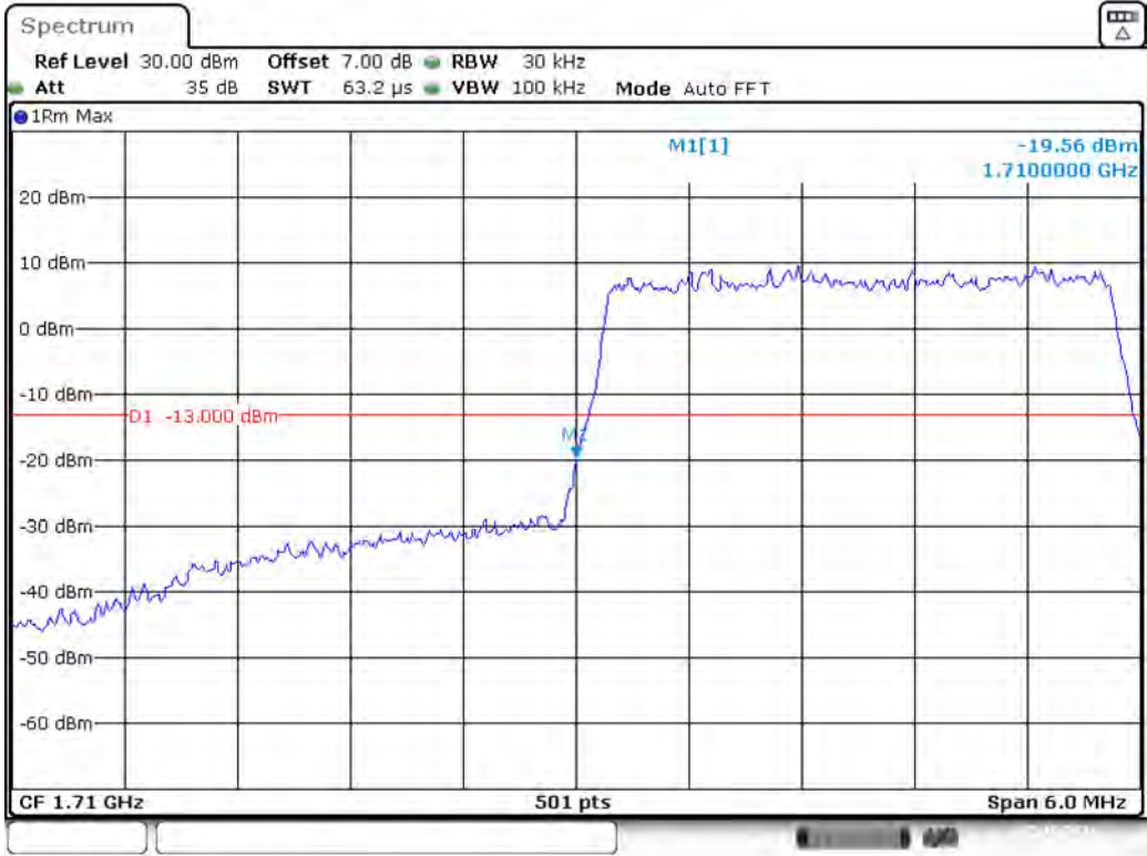
Band 4_3 MHz_Low_16QAM_RB15#0
