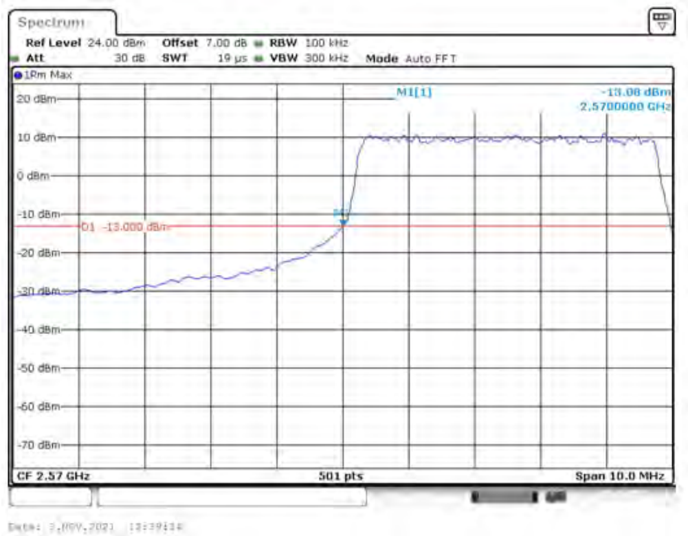
Band 38_5 MHz_Low_16QAM_RB25#0
