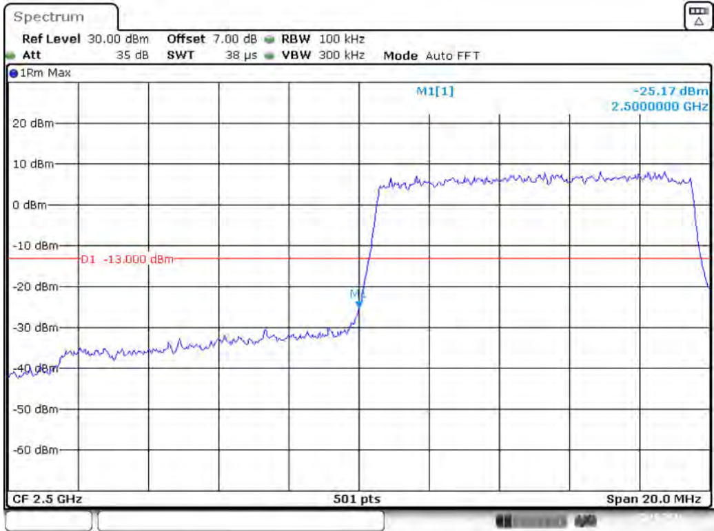
Band 7_10 MHz_Low_QPSK_RB50#0
