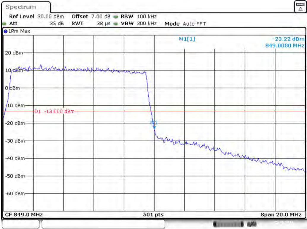
Band 5_10 MHz_High_16QAM_RB50#0
