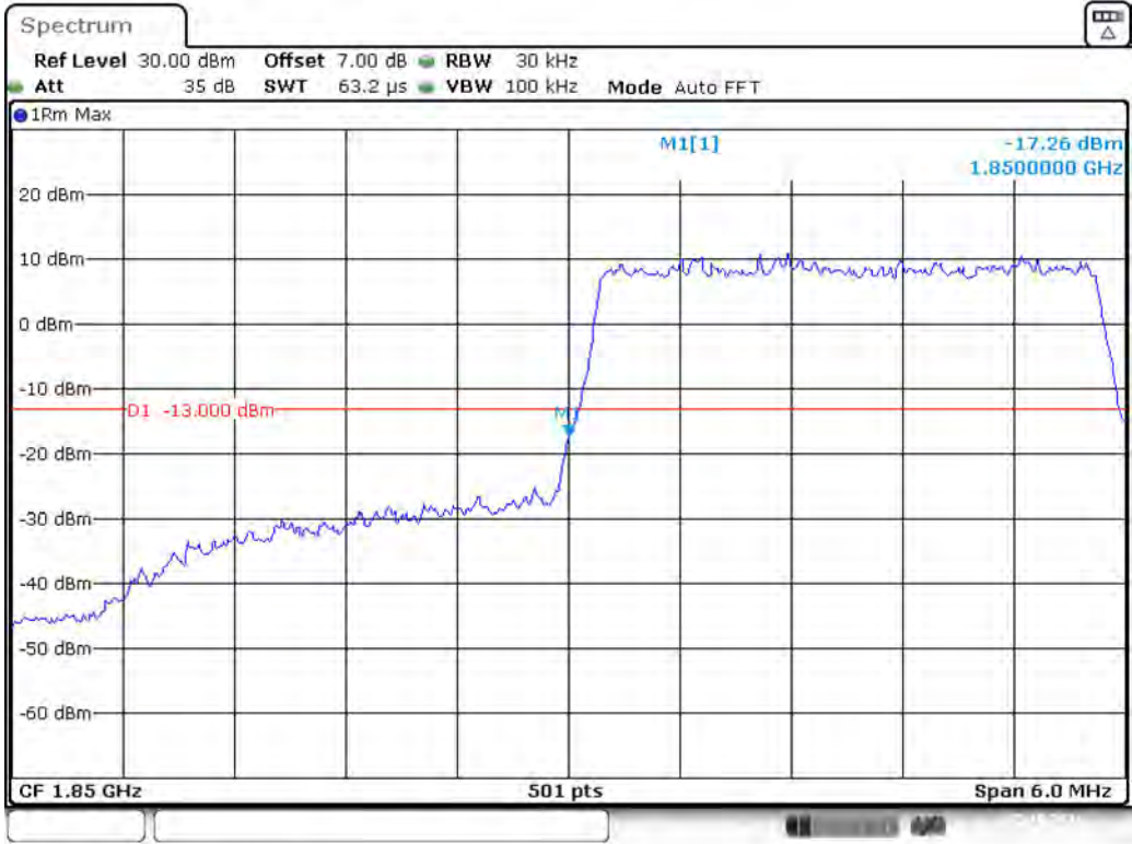
Band 2_3 MHz_Low_16QAM_RB15#0
