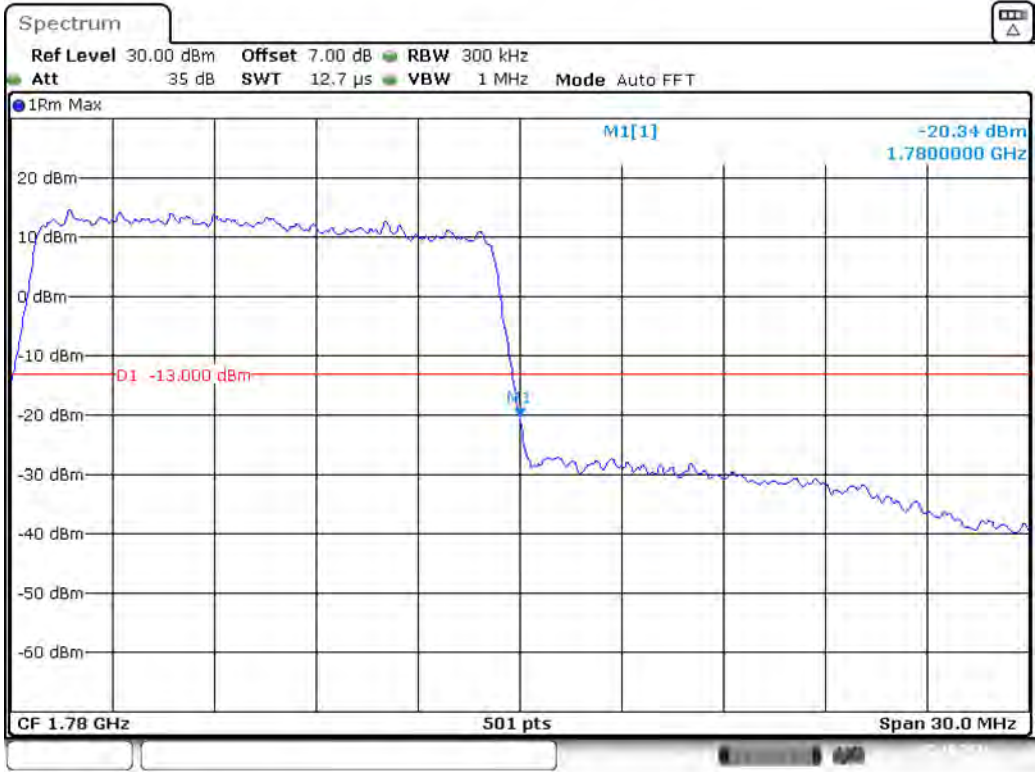
Band 66_15 MHz_High_16QAM_RB75#0
