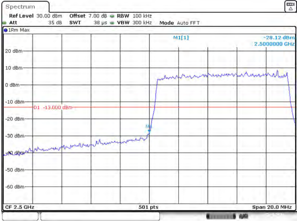
Band 7_10 MHz_Low_16QAM_RB50#0
