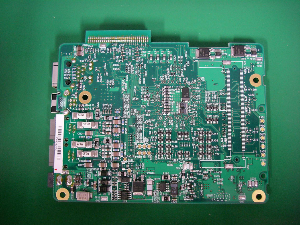
11. BB board(back view)
