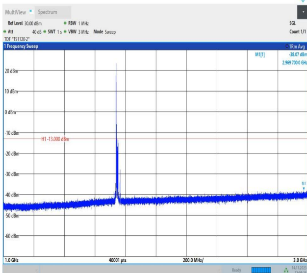
Band66_15MHz_16QAM_132322_1RB#0_1000~3000_1000~3000
