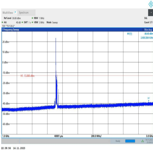
Band66_20MHz_16QAM_132072_1RB#0_1000~3000_1000~3000
