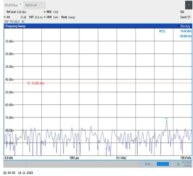
Band66_20MHz_16QAM_132322_1RB#0_0.009~0.15_0.009~0.15
