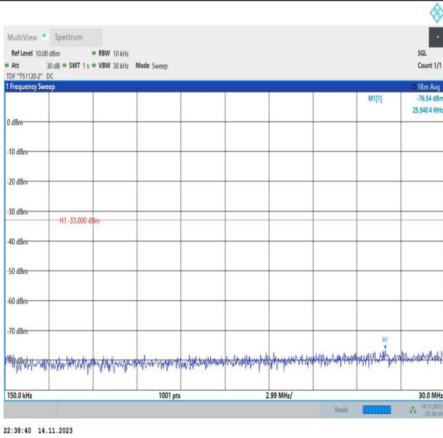
Band66_20MHz_16QAM_132072_1RB#0_0.15~30_0.15~30
