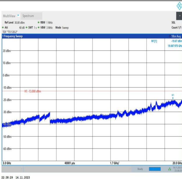
Band66_20MHz_QPSK_132072_1RB#0_3000~20000_3000~20000
