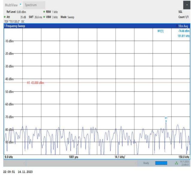
Band66_15MHz_16QAM_132597_1RB#0_0.009~0.15_0.009~0.15
