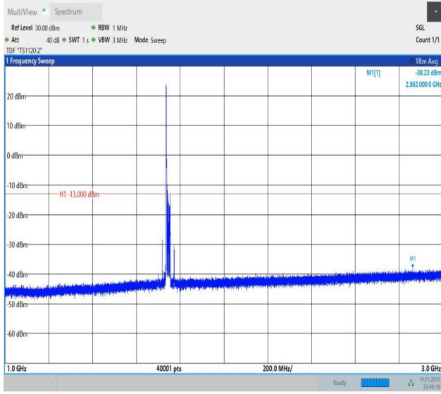
Band66_20MHz_16QAM_132322_1RB#0_1000~3000_1000~3000
