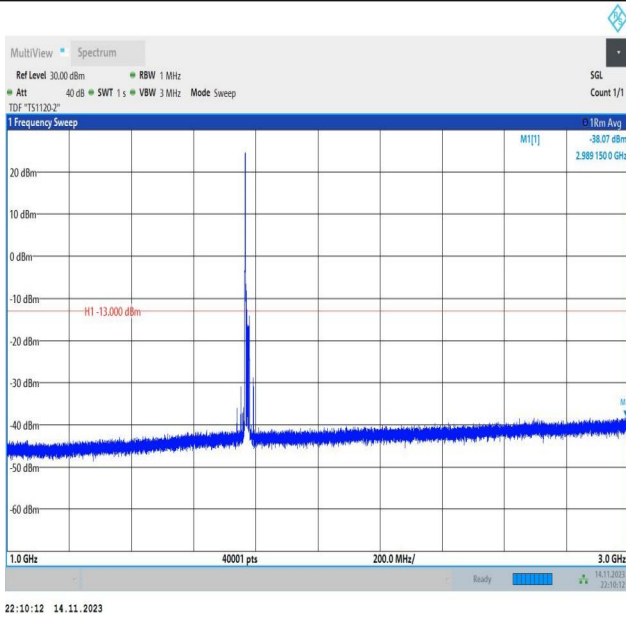
Band66_15MHz_16QAM_132597_1RB#0_1000~3000_1000~3000
