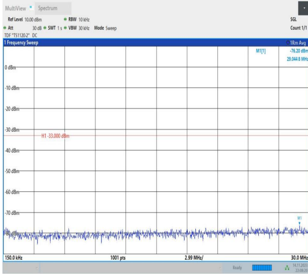
Band66_15MHz_16QAM_132322_1RB#0_0.15~30_0.15~30
