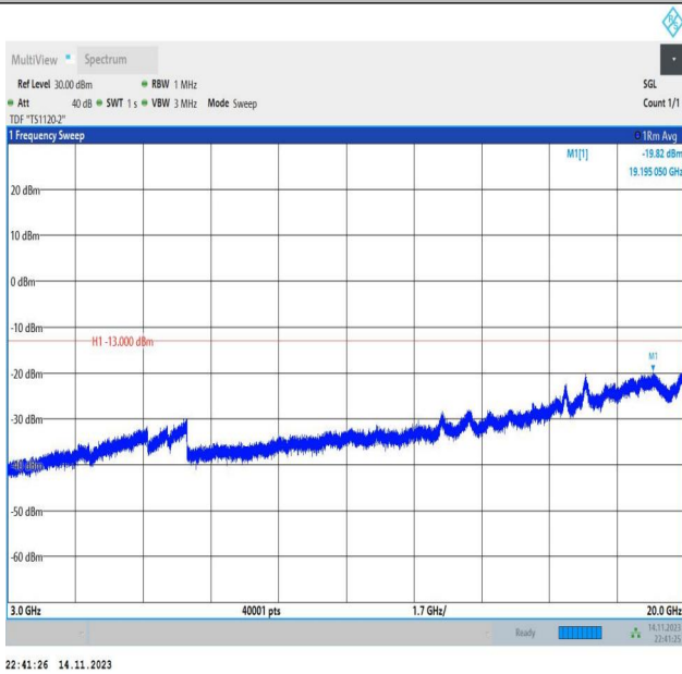
Band66_20MHz_QPSK_132572_1RB#0_3000~20000_3000~20000
