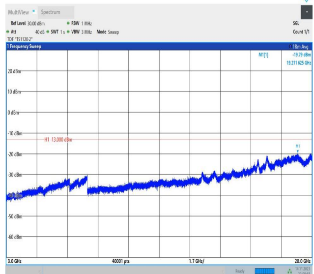
Band66_15MHz_16QAM_132322_1RB#0_3000~20000_3000~20000
