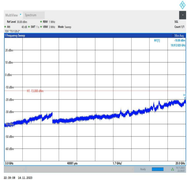
Band66_20MHz_16QAM_132072_1RB#0_3000~20000_3000~20000
