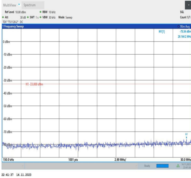
Band66_20MHz_16QAM_132572_1RB#0_0.15~30_0.15~30
