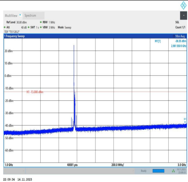
Band66_15MHz_QPSK_132597_1RB#0_1000~3000_1000~3000
