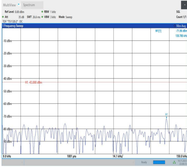
Band66_15MHz_QPSK_132597_1RB#0_0.009~0.15_0.009~0.15
