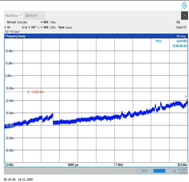
Band66_15MHz_16QAM_132597_1RB#0_3000~20000_3000~20000
