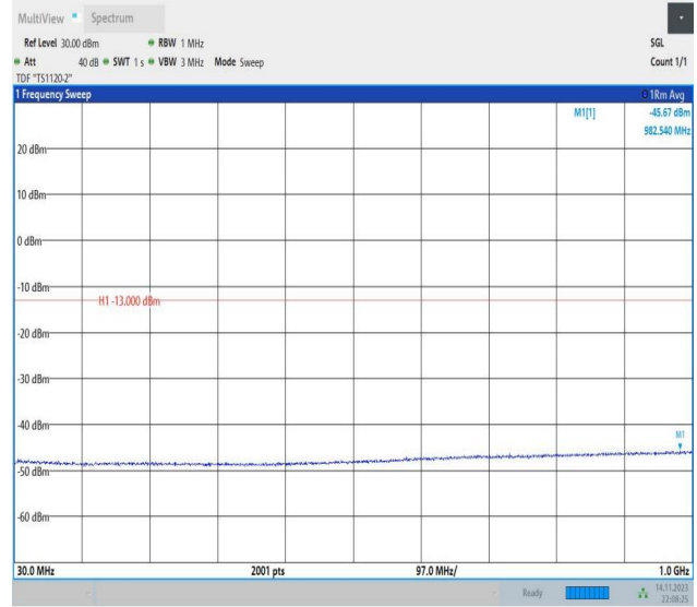
Band66_15MHz_16QAM_132322_1RB#0_30~1000_30~1000
