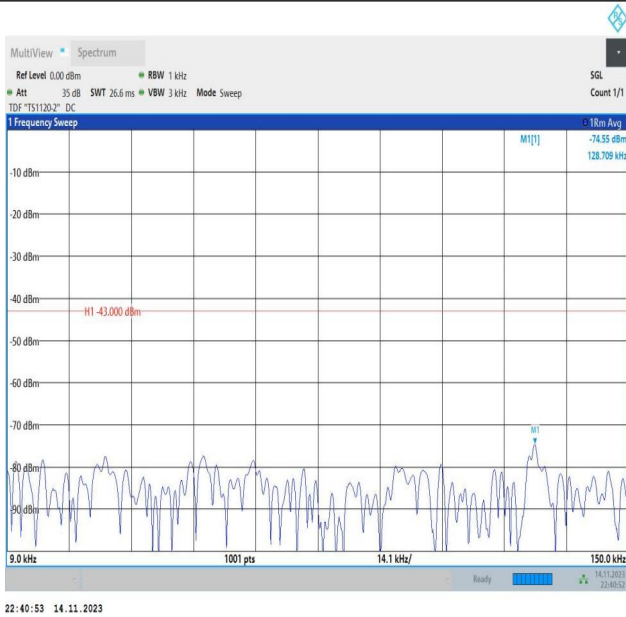
Band66_20MHz_QPSK_132572_1RB#0_0.009~0.15_0.009~0.15
