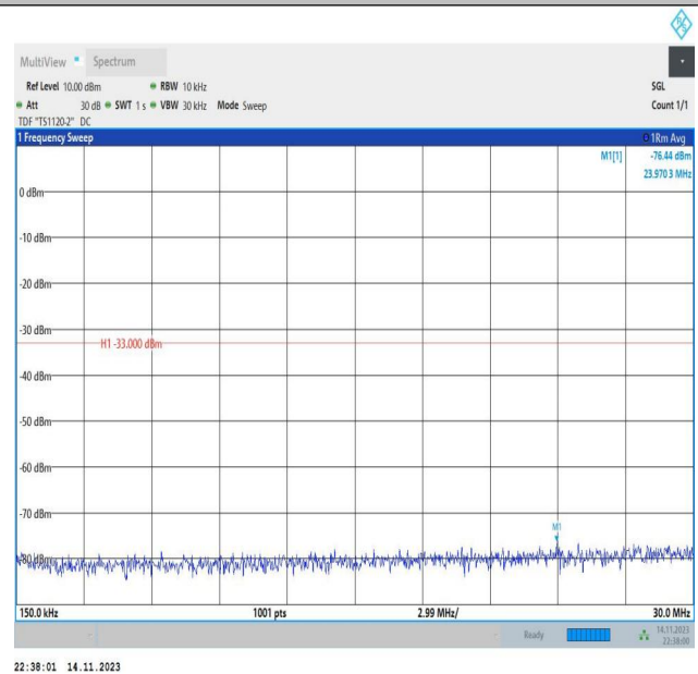
Band66_20MHz_QPSK_132072_1RB#0_0.15~30_0.15~30
