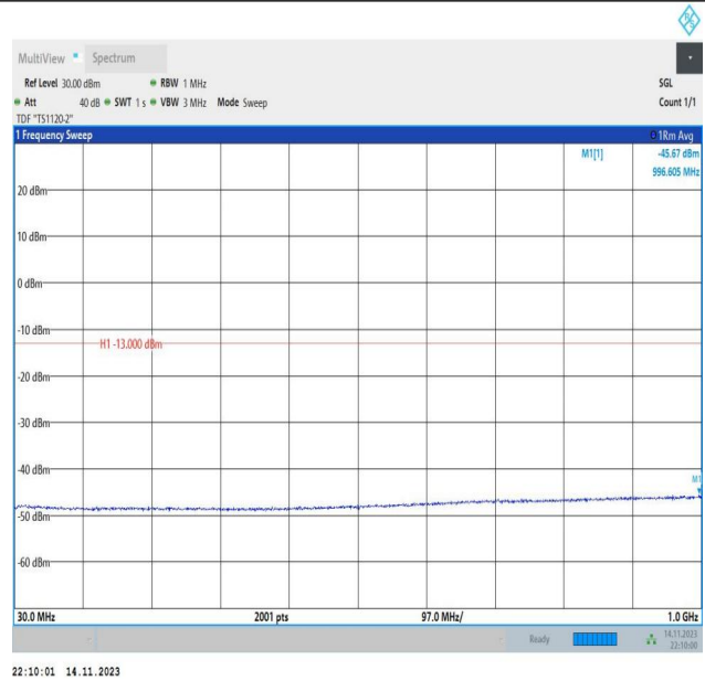
Band66_15MHz_16QAM_132597_1RB#0_30~1000_30~1000
