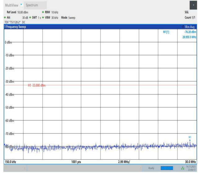
Band66_15MHz_QPSK_132597_1RB#0_0.15~30_0.15~30
