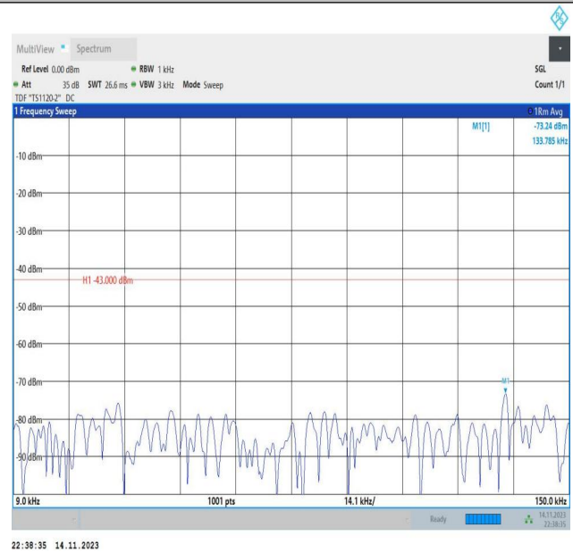
Band66_20MHz_16QAM_132072_1RB#0_0.009~0.15_0.009~0.15
