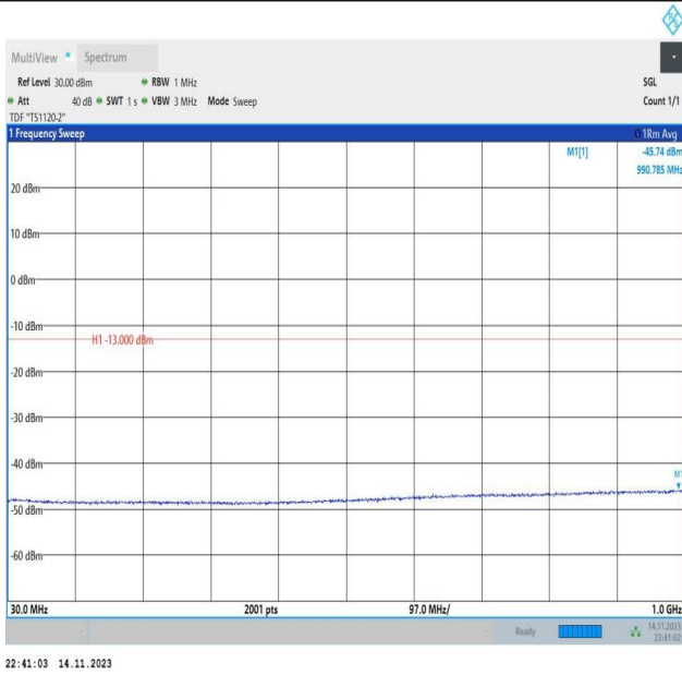
Band66_20MHz_QPSK_132572_1RB#0_30~1000_30~1000
