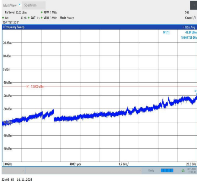
Band66_15MHz_QPSK_132597_1RB#0_3000~20000_3000~20000
