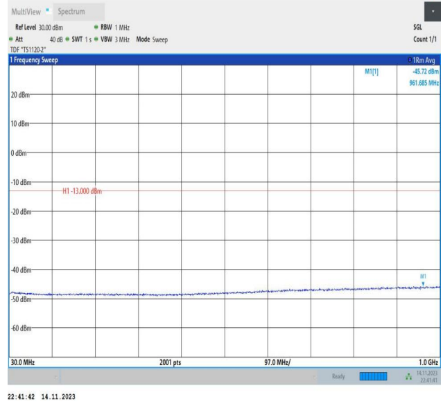
Band66_20MHz_16QAM_132572_1RB#0_30~1000_30~1000
