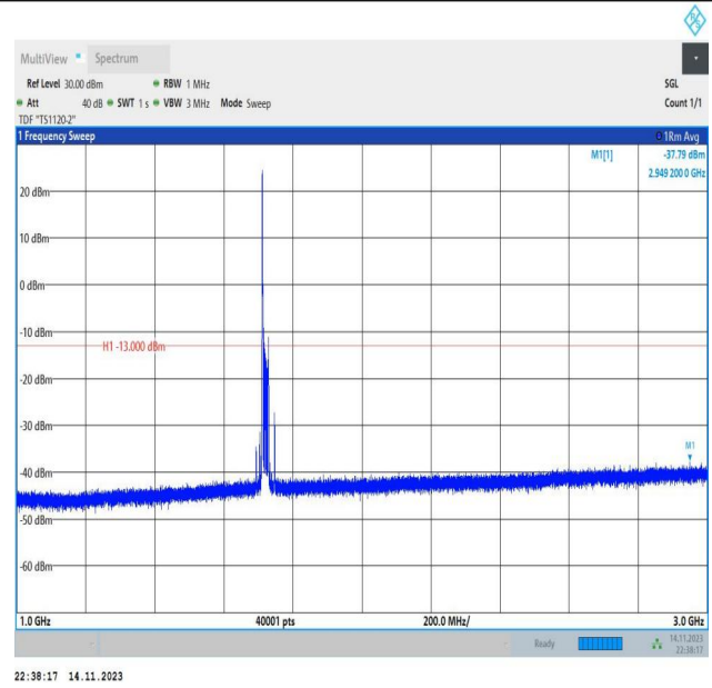
Band66_20MHz_QPSK_132072_1RB#0_1000~3000_1000~3000
