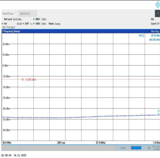
Band66_20MHz_QPSK_132072_1RB#0_30~1000_30~1000
