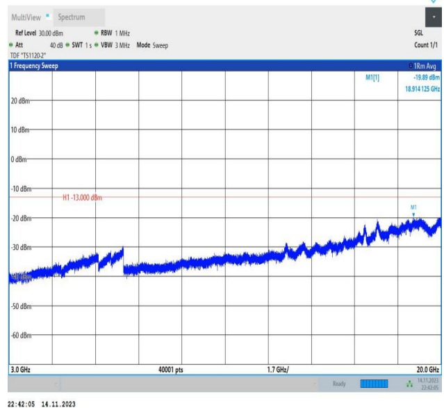
Band66_20MHz_16QAM_132572_1RB#0_3000~20000_3000~20000
