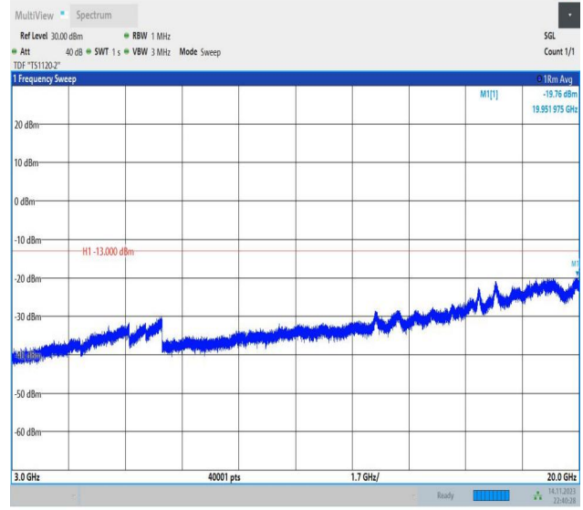
Band66_20MHz_16QAM_132322_1RB#0_3000~20000_3000~20000
