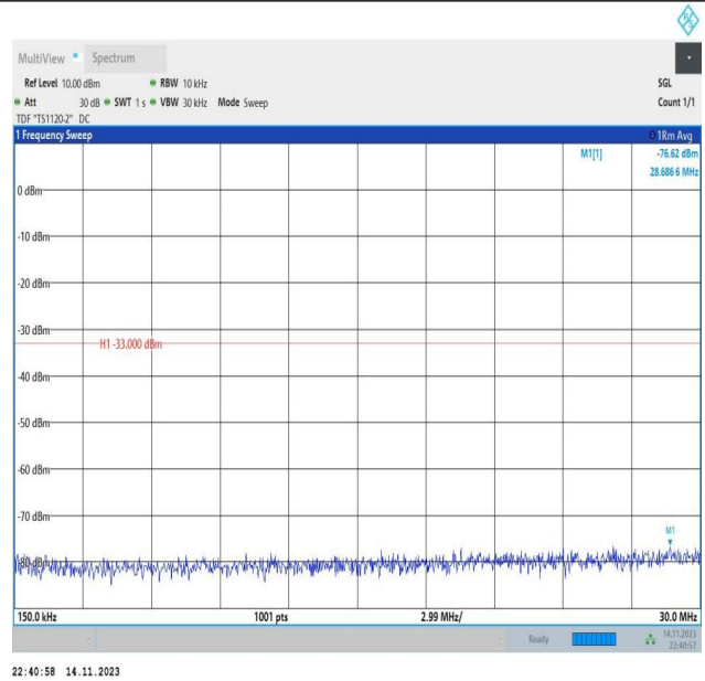
Band66_20MHz_16QAM_132322_1RB#0_3000~20000_3000~20000
