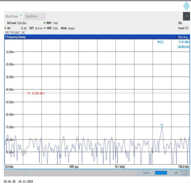
Band66_20MHz_16QAM_132572_1RB#0_0.009~0.15_0.009~0.15
