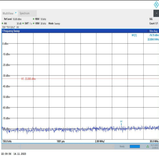
Band66_15MHz_16QAM_132597_1RB#0_0.15~30_0.15~30
