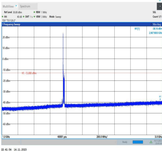
Band66_20MHz_16QAM_132572_1RB#0_1000~3000_1000~3000
