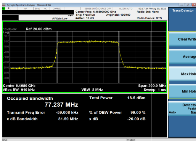
Plot 7-29. 26dB & 99% Bandwidth Plot Antenna WF5t (80MHz 802.11ax (UNII Band 6) – Ch. 103, MCS4)
