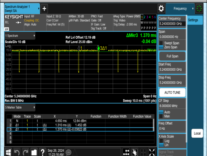
NTNV-11AC20SISO-Ant2-5240
