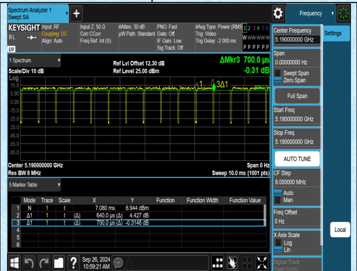
NTNV-11N40SISO-Ant2-5190
