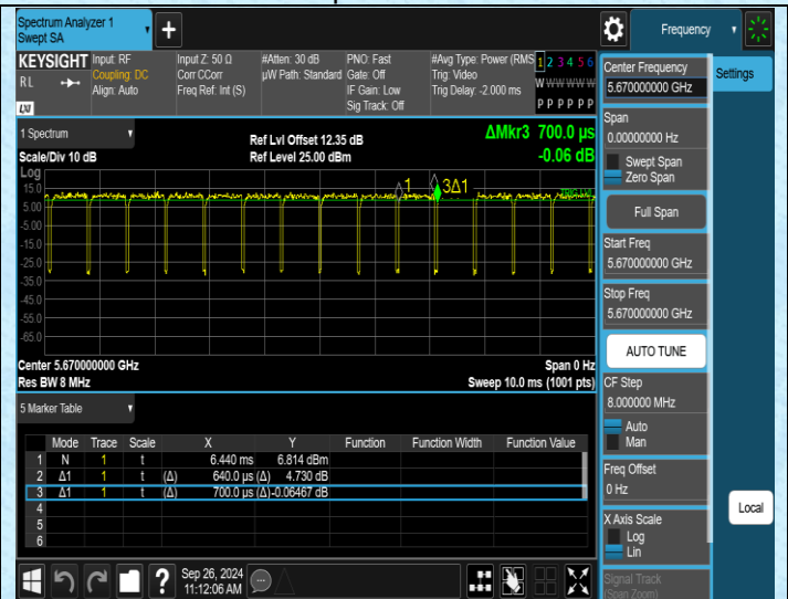
NTNV-11N40SISO-Ant2-5670
