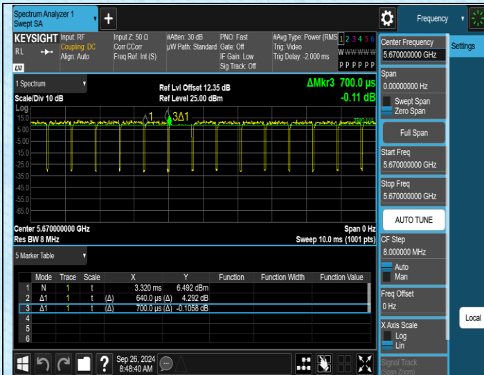
NTNV-11N40SISO-Ant1-5670
