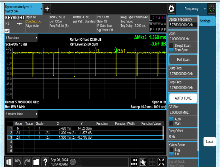
NTNV-11N20SISO-Ant2-5785
