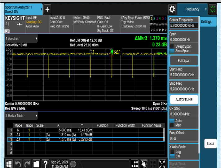
NTNV-11AC20SISO-Ant2-5700
