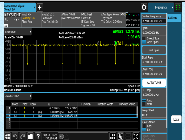
NTNV-11AC20SISO-Ant2-5580
