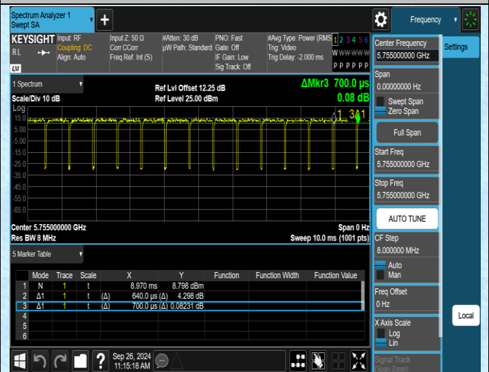
NTNV-11N40SISO-Ant2-5755
