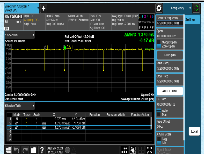
NTNV-11AC20SISO-Ant2-5200
