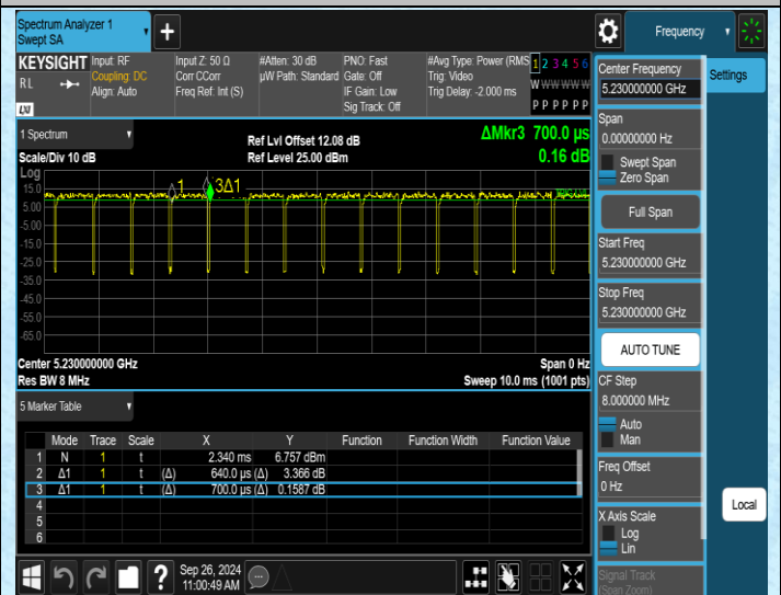
NTNV-11N40SISO-Ant2-5230
