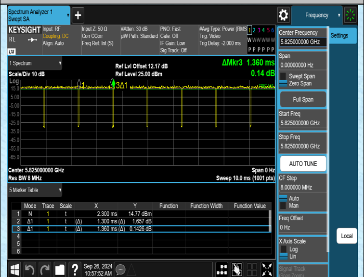
NTNV-11N20SISO-Ant2-5825
