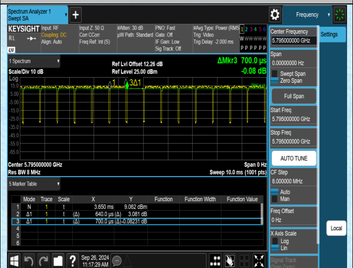
NTNV-11N40SISO-Ant2-5795
