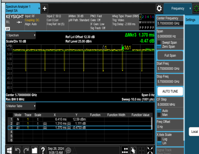
NTNV-11AC20SISO-Ant1-5700
