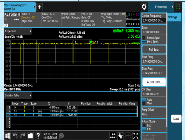
NTNV-11N20SISO-Ant2-5745
