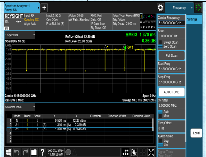
NTNV-11AC20SISO-Ant2-5180
