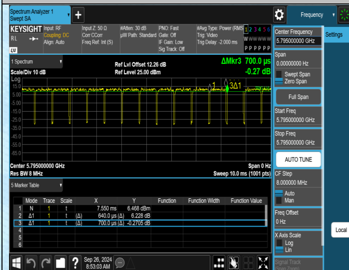
NTNV-11N40SISO-Ant1-5795
