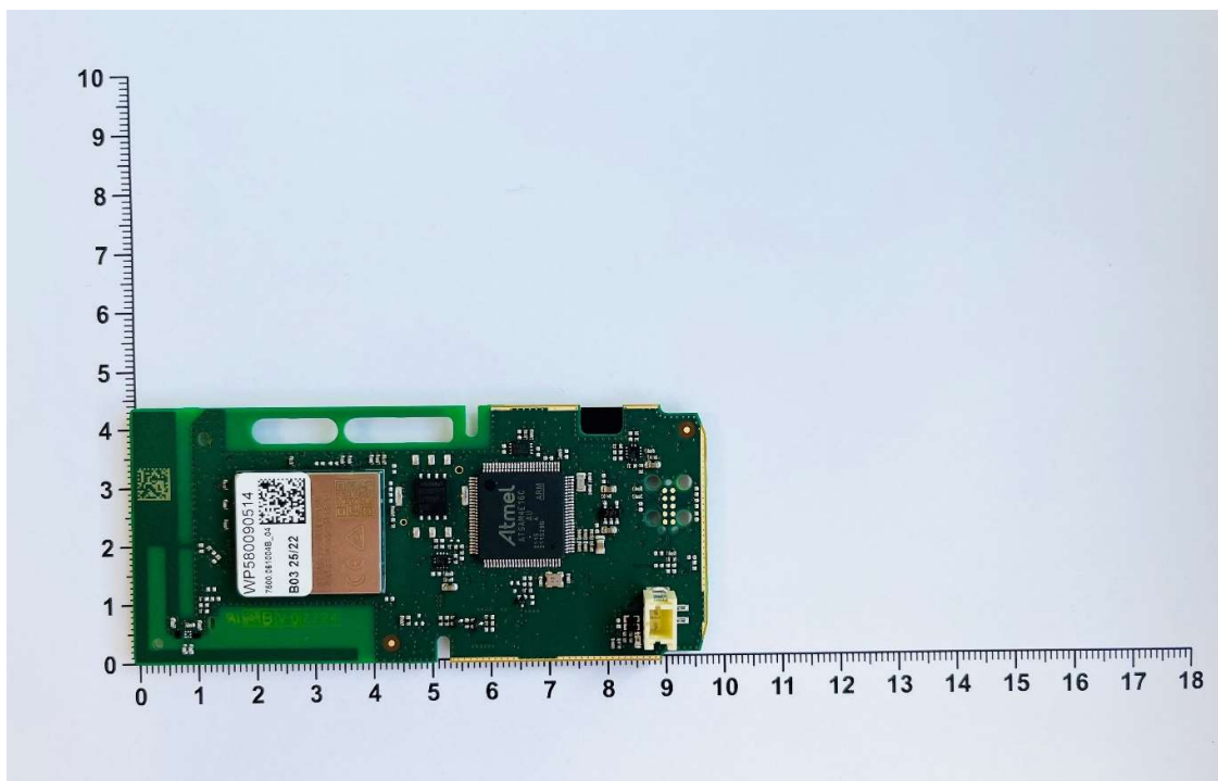
TU600-21 Print seen from the top
