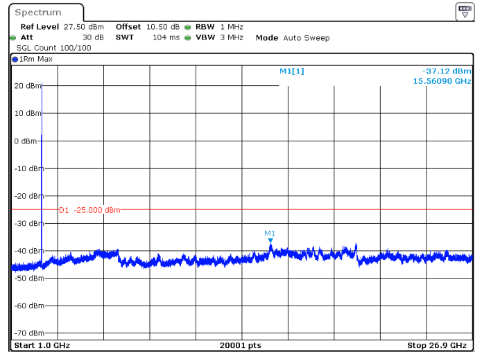
20MHz_15kHz_2679.99MHz_DFT-s-OFDM QPSK_RB1@105 -37.12 dBm
