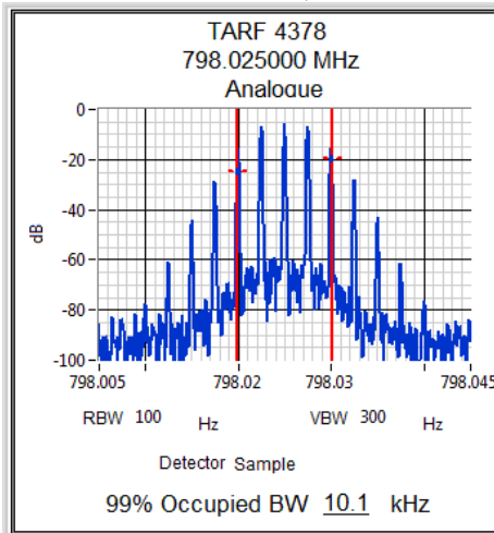
798.025 MHz, 3 W
