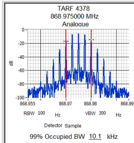
868.975 MHz, 3 W
