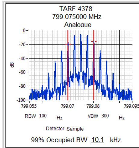
799.075 MHz, 3 W
