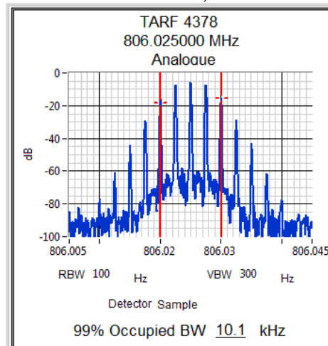
806.025 MHz, 3 W
