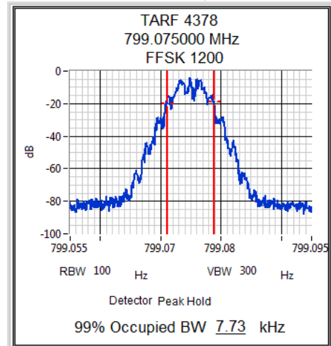
799.075 MHz, 3 W
