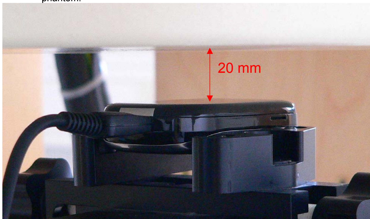
Fig. 39: Body worn configuration, GPRS (Class 8) with data cable, slider down, antenna towards the phantom.
