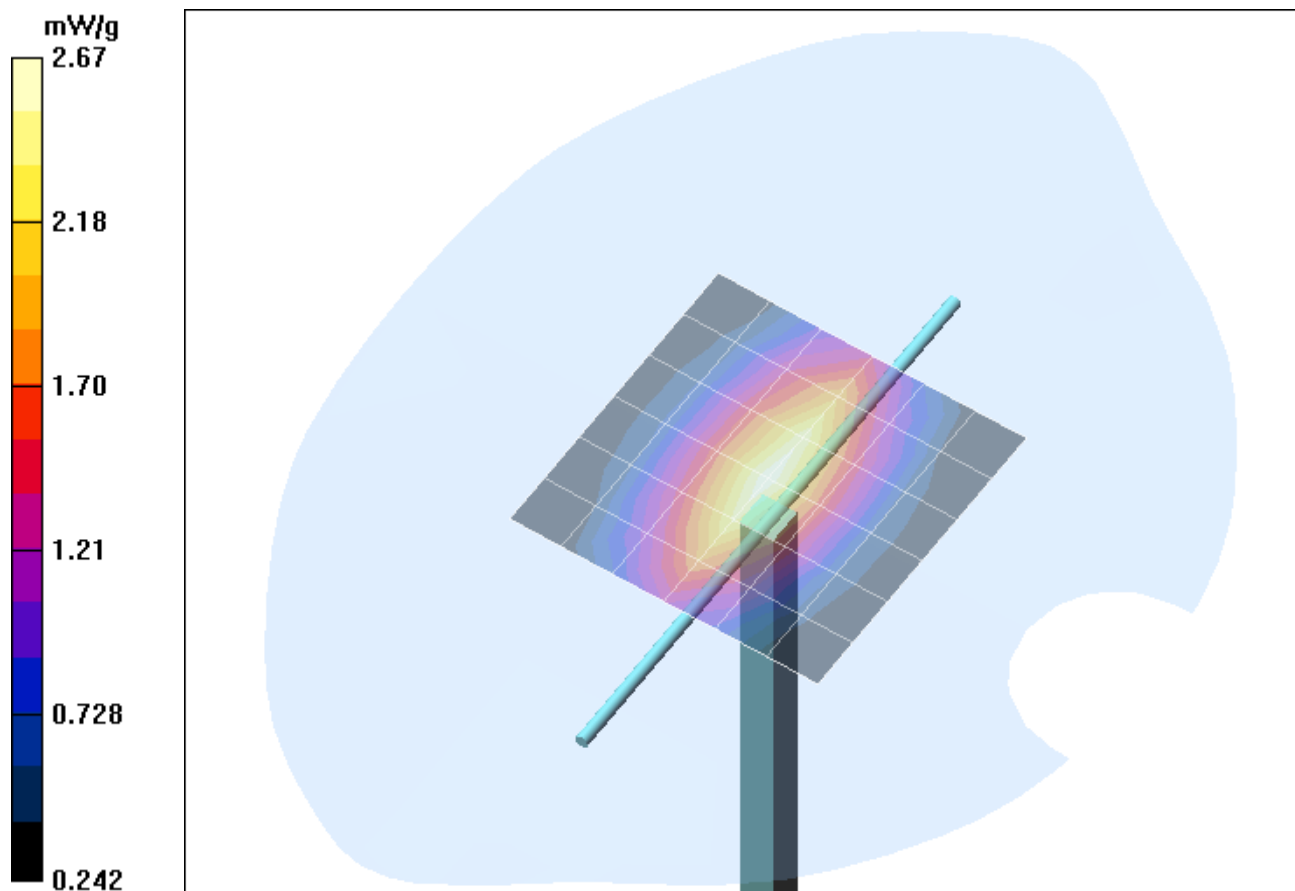
Fig. 12: Validation measurement 835 MHz Head (March 24, 2006), coarse grid. Ambient Temperature: 22.0° C, Liquid Temperature: 21.0° C.
