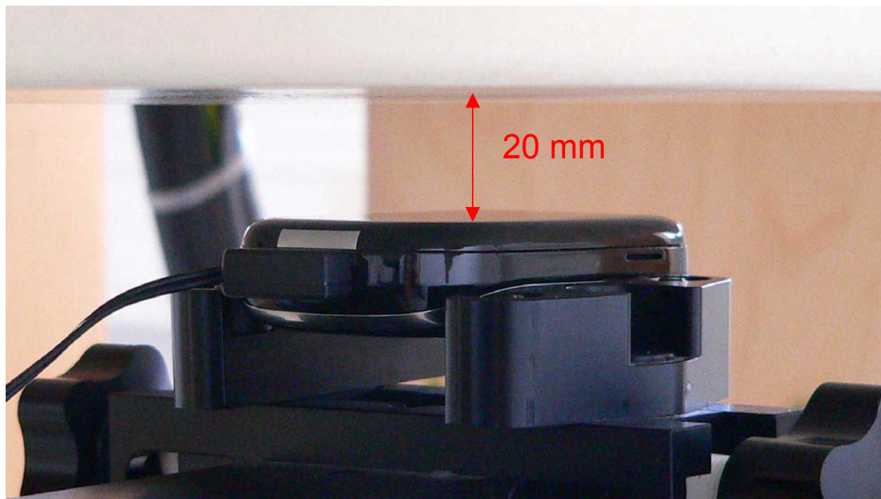
Fig. 38: Body worn configuration, GSM with headset, slider down, antenna towards the phantom.
