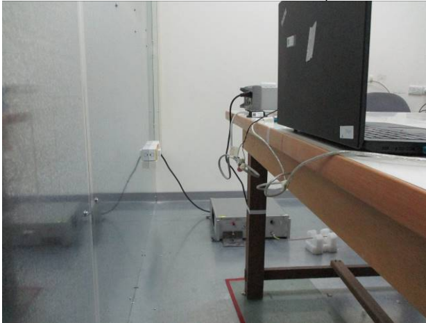
FCC_15_247_BLE_Conduction_Setup
