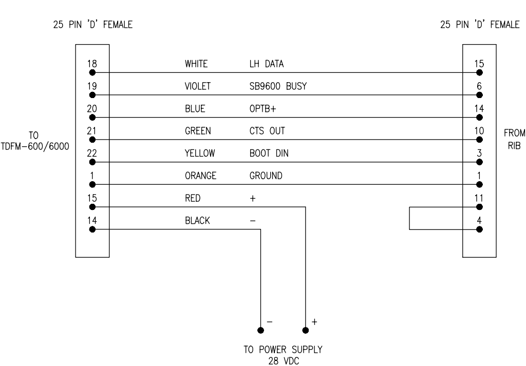
FIGURE 2-2 Type I (XTS-3000) Programming Cable (Requires RIB)
