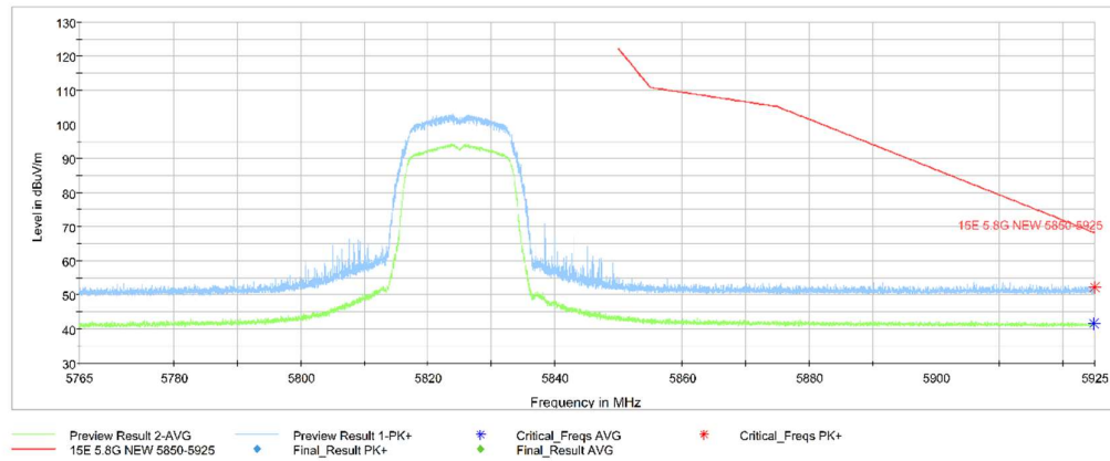
Fig. 2 Band Edges (802.11a Ch165, 5825MHz)
