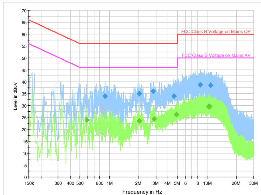
Fig.A.6.1. AC Powerline Conducted Emission-802.11a CH149
