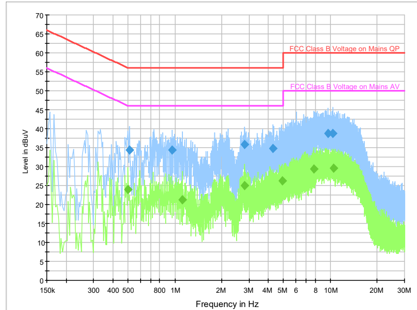
Fig.A.6.2. AC Powerline Conducted Emission-Idle
