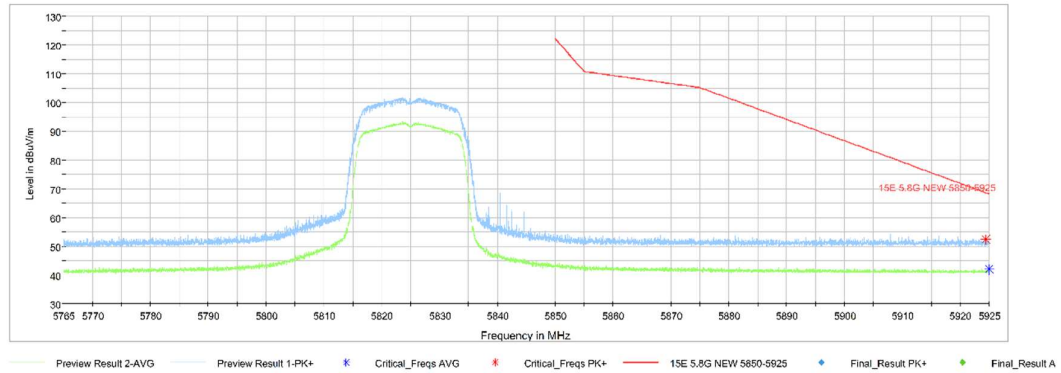
Fig. 8 Band Edges (802.11ac-HT20 Ch165, 5825MHz)
