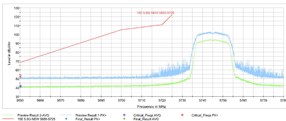
Fig. 1 Band Edges (802.11a Ch149,5745MHz)
