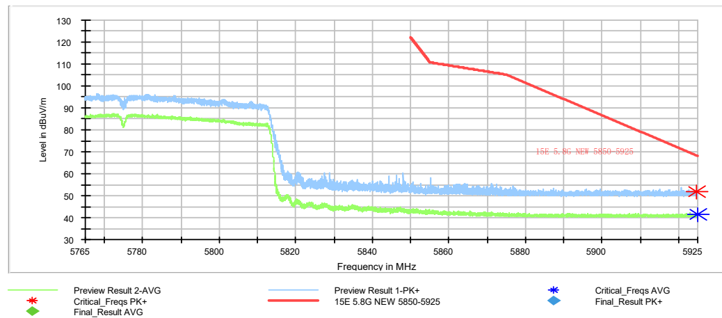
Fig. 12 Band Edges (802.11ac-HT80, 5775MHz)
