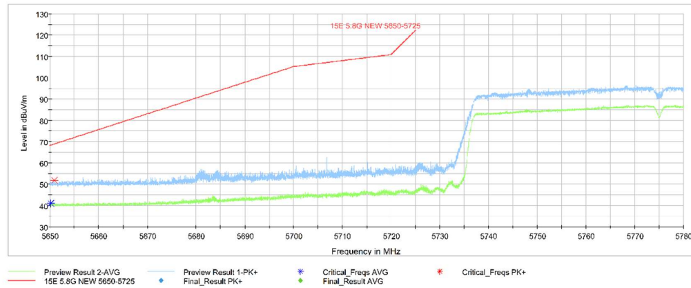
Fig. 11 Band Edges (802.11ac-HT80 Ch155, 5775MHz)
