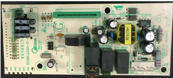
Original Mother board-top view
