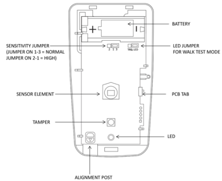
Figure 3: PCB layout
