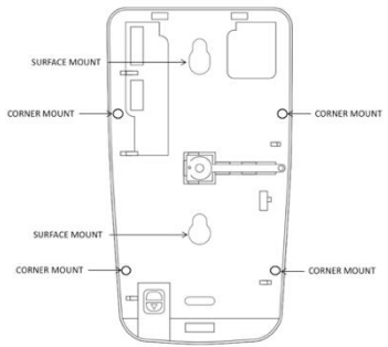
Figure 4: Mounting locations
