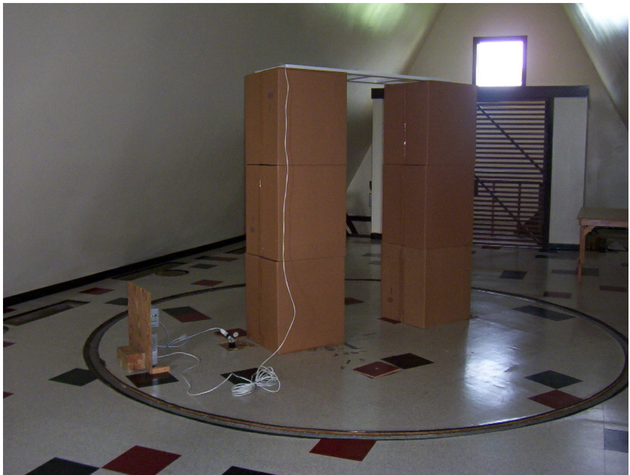
Photo 2 – Rear View of Radiated Emissions Setup
