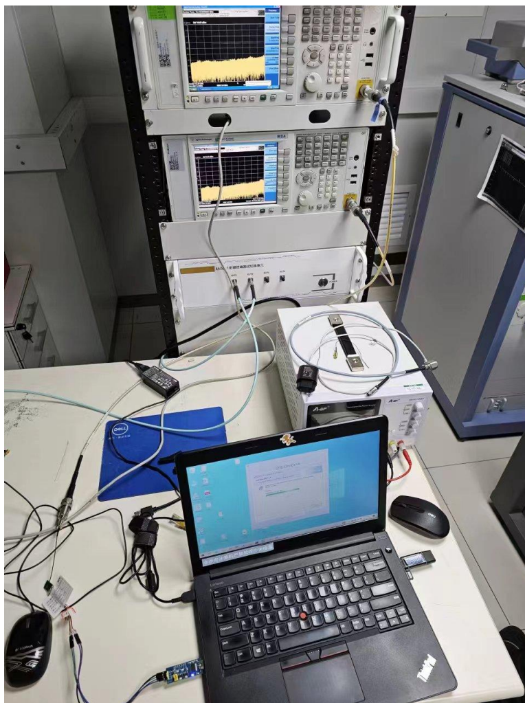
RF Conducted Test setup (BLE)
