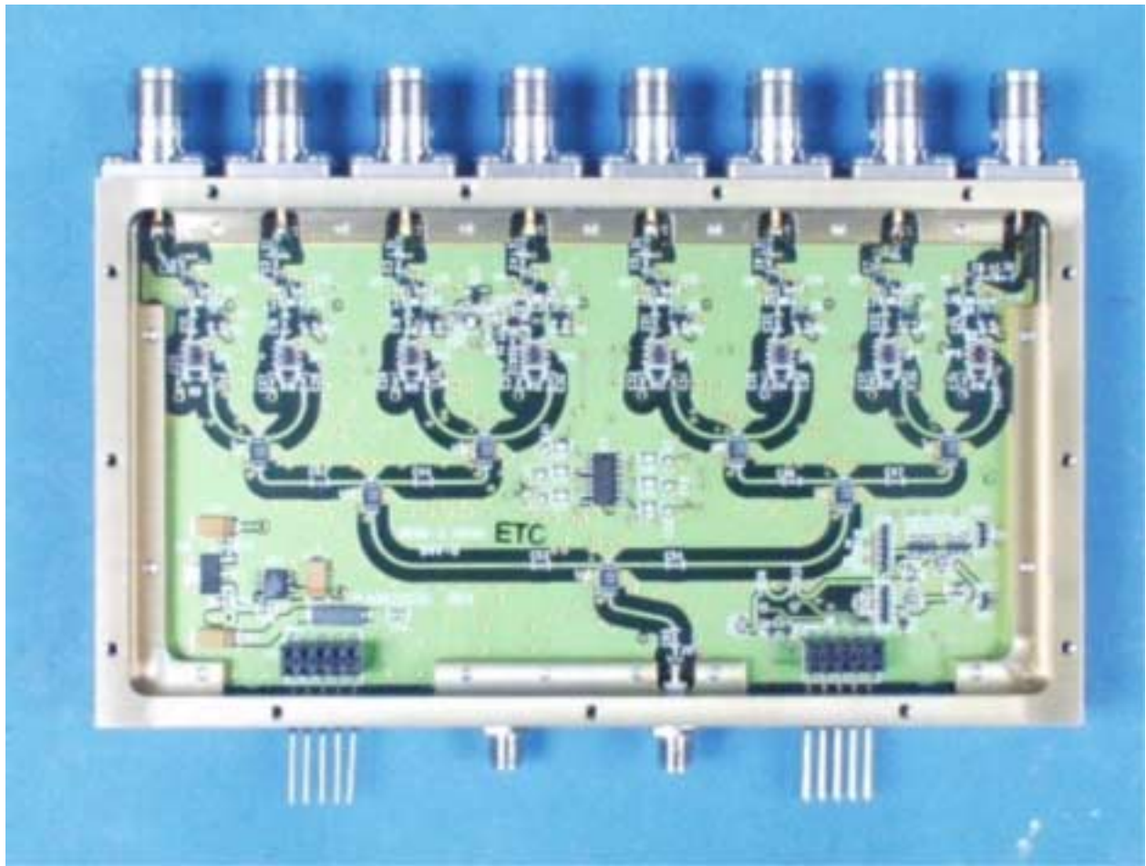
Multiplexer, Bottom
