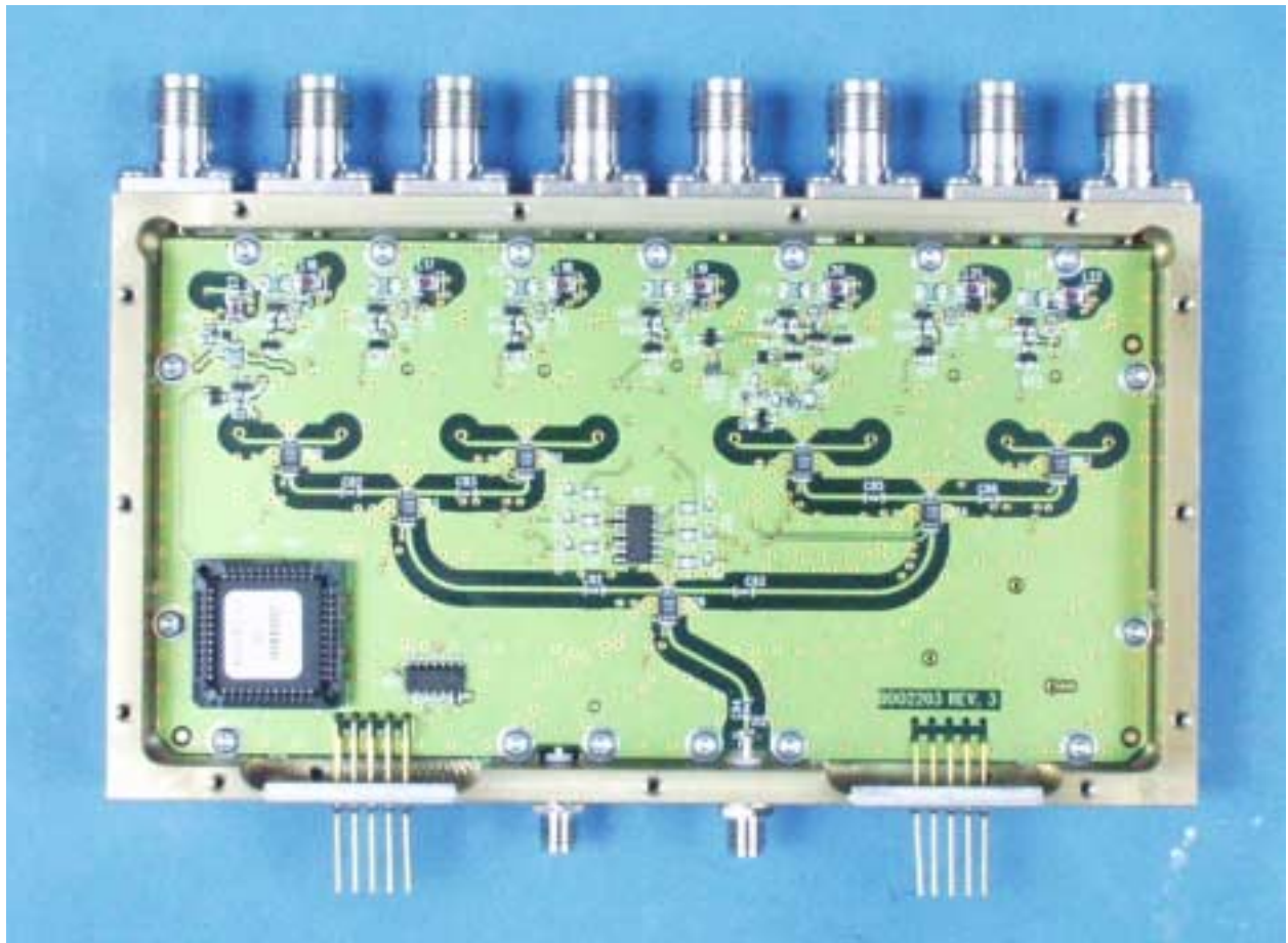
Multiplexer, Top
