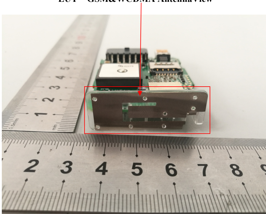
EUT – GSM&WCDMA AntennaView
