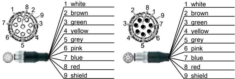
Fig. 18: Colour coding example: M12x1 socket / connector, A coded, 8 pin, shielded
