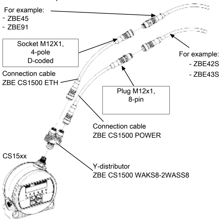
Fig. 14: Connection example CS15xx-0-...
