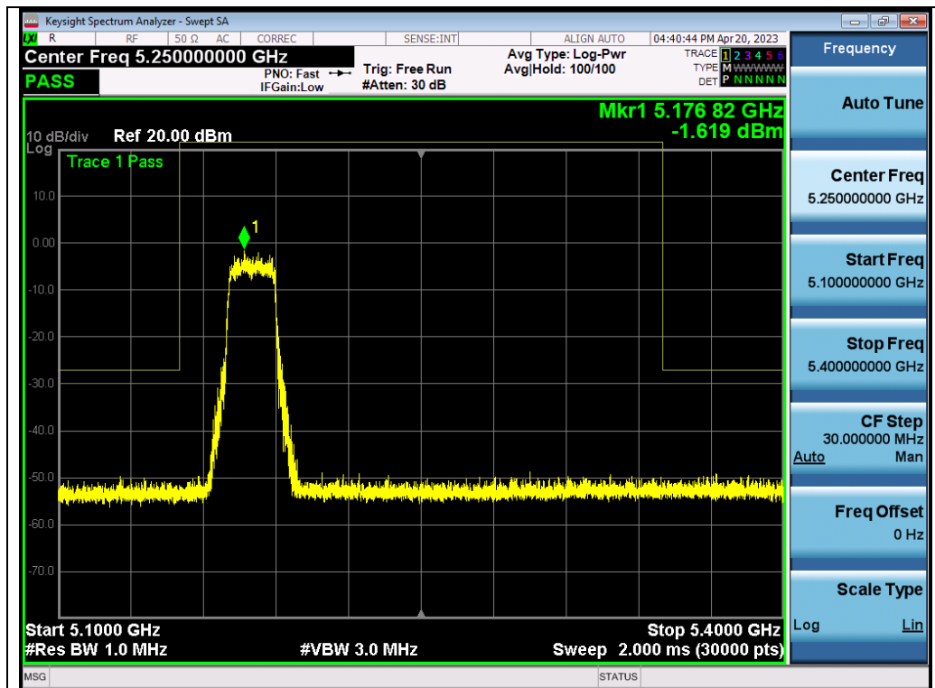
Test_Graph_802.11ax20_ANT2_5180_MCS0_Frequency Band 3
