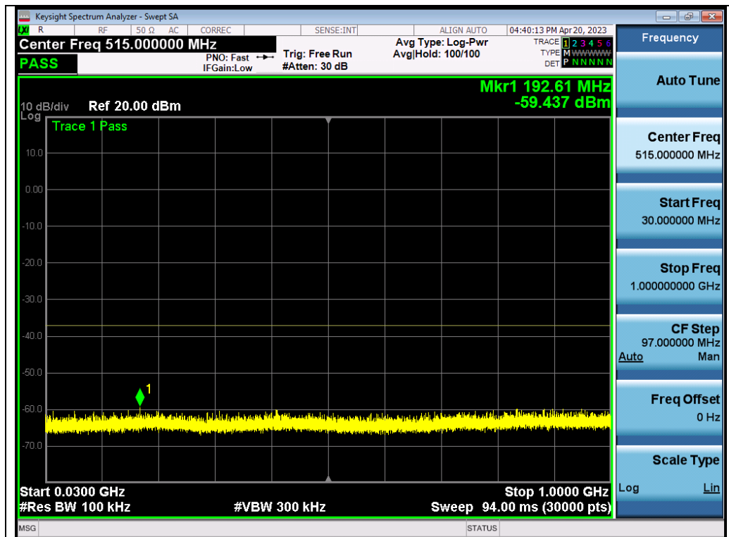
Test_Graph_802.11ax20_ANT2_5180_MCS0_Frequency Band 1
