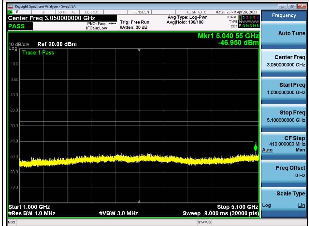
Test_Graph_802.11ax20_ANT1_5180_MCS0_Frequency Band 2
