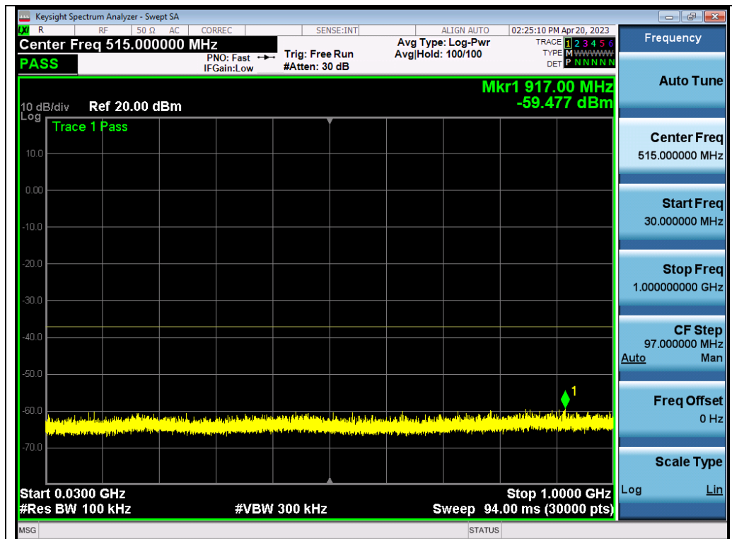
Test_Graph_802.11ax20_ANT1_5180_MCS0_Frequency Band 1
