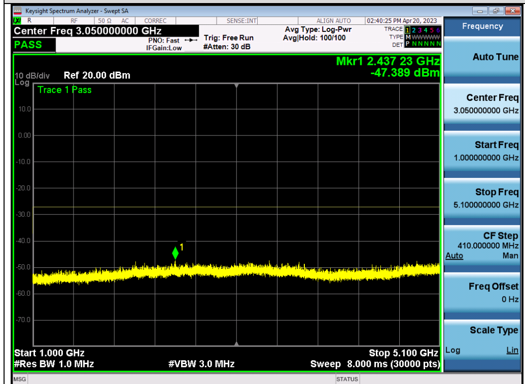
Test_Graph_802.11ax80_ANT1_5210_MCS0_Frequency Band 2
