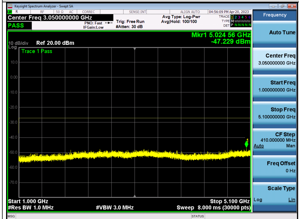
Test_Graph_802.11ax80_ANT2_5210_MCS0_Frequency Band 2
