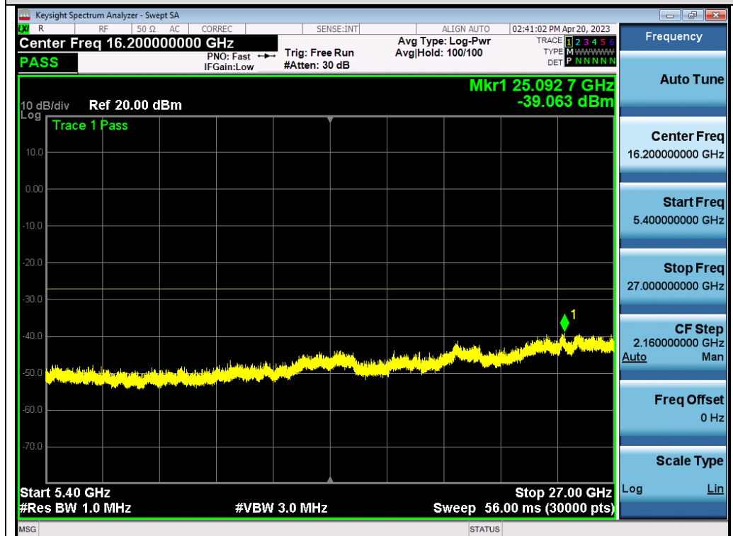
Test_Graph_802.11ax80_ANT1_5210_MCS0_Frequency Band 4
