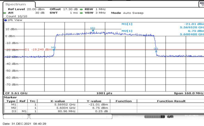
11AX80MIMO Ant2 5610
