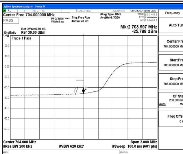
Band17-10MHz-16QAM-23800-50RB#0
