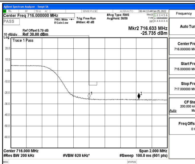
Band17-10MHz-16QAM-23780-50RB#0
