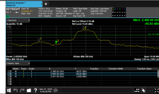
Out Of Band Emission π/4DQPSK_2-DH5_Channel 0
