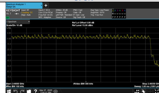
High End Spectrum Channel Hopping Plot \pi/4 DQPSK
