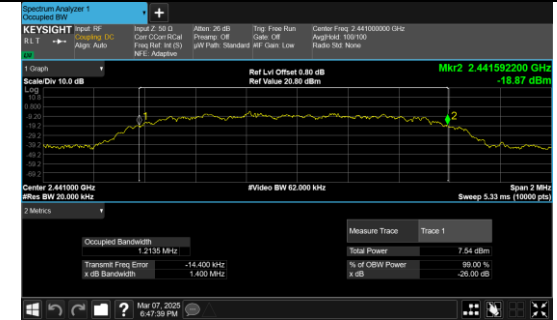
\pi/4 DQPSK 2-DH5 Channel 39
