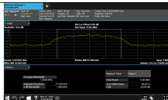
8DPSK_3-DH5_Channel 39
