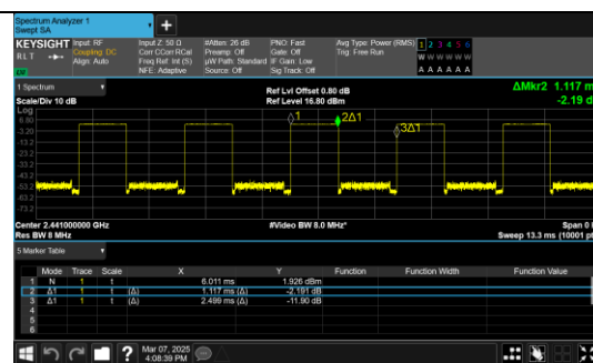
GFSK(DH5)_Channel 39
