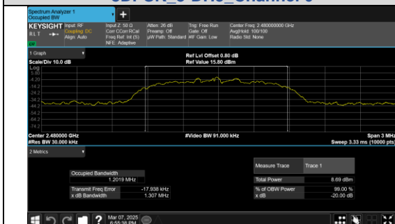
8DPSK_3-DH5_Channel 78
