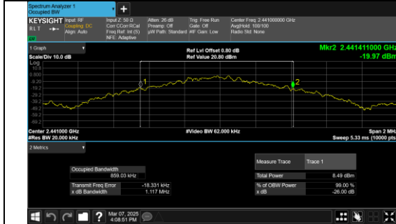
GFSK DH5 Channel 39
