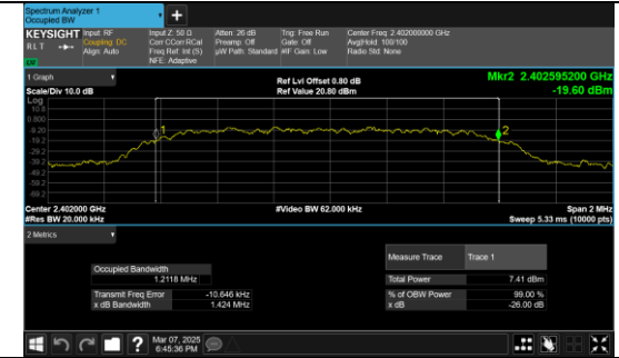
\pi/4 DQPSK 2-DH5 Channel 0
