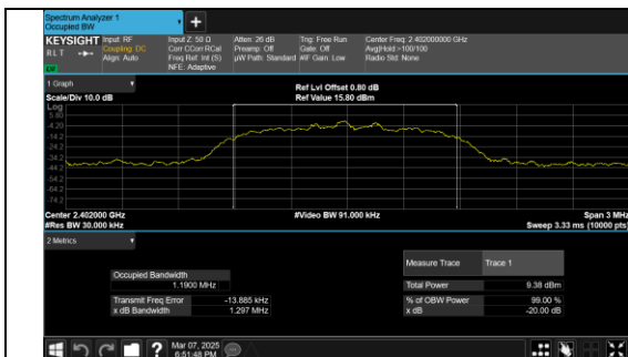
8DPSK_3-DH5_Channel 0
