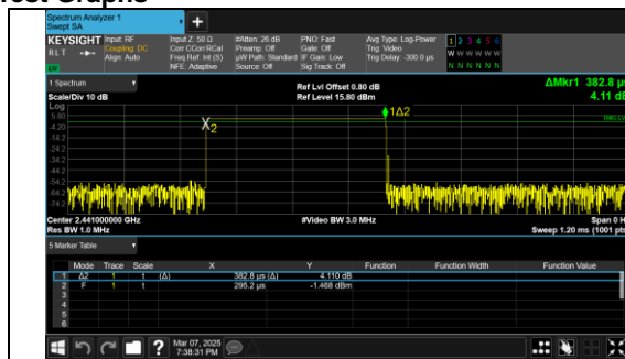
Pulse Width GFSK DH1
