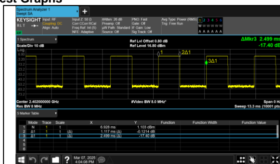
GFSK(DH5)_Channel 0
