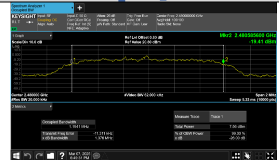
\pi/4 DQPSK 2-DH5 Channel 78
