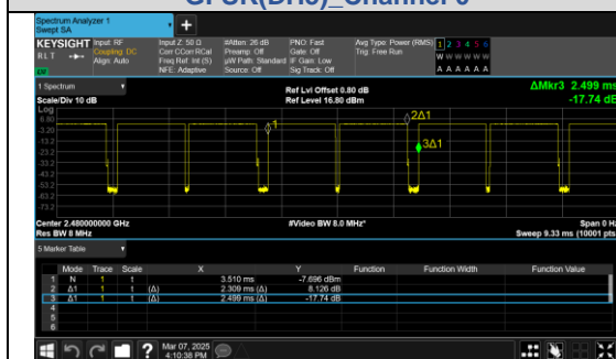
GFSK(DH5)_Channel 78
