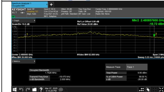
GFSK DH5 Channel 78
