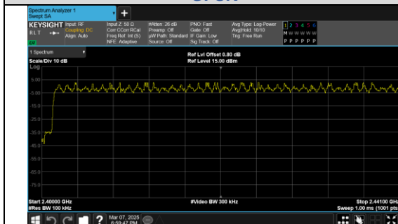
Low End Spectrum Channel Hopping Plot \pi/4 DQPSK
