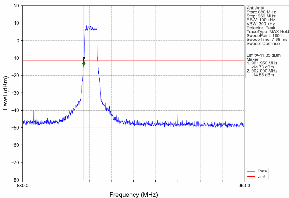
5M_LCH_904.6MHz_Ant0_NTNV
