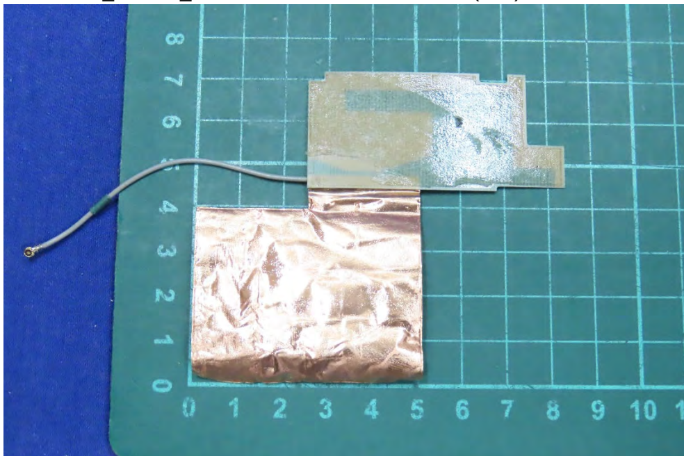
(31) EUT Photo_WWAN_SPEED/F-0G-MA-6001-002-00(Aux)
