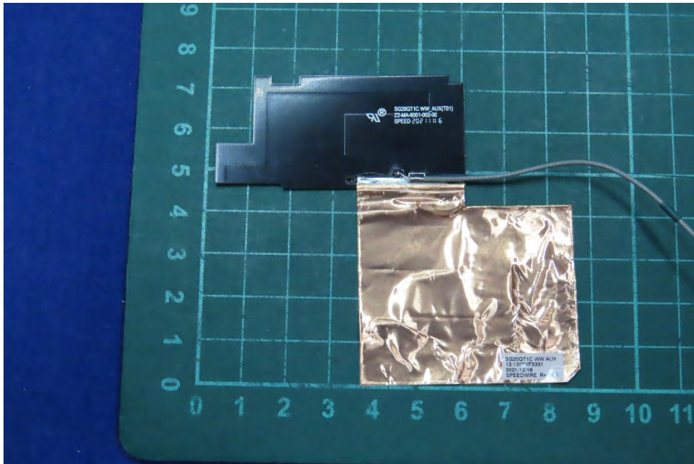
(30) EUT Photo_WWAN_SPEED/F-0G-MA-6001-002-00(Aux)
