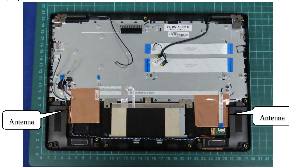
(26) EUT Photo
