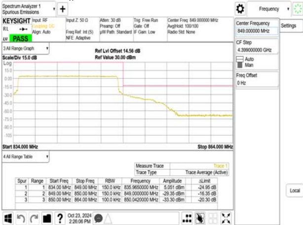
Band Edge_Band26_15MHz_OPSK_RB75_0_CH26965
