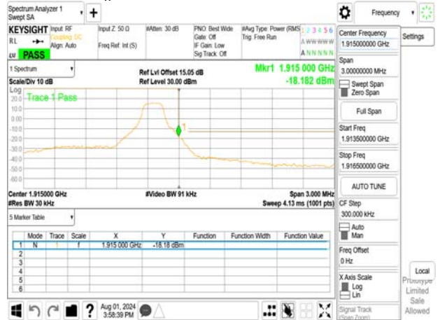
Band Edge_Band25_1.4MHz_OPSK_RB1_5_CH26683
