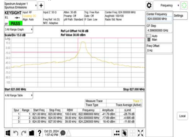
Band Edge_Band26_3MHz_OPSK_RB1_0_CH26805
