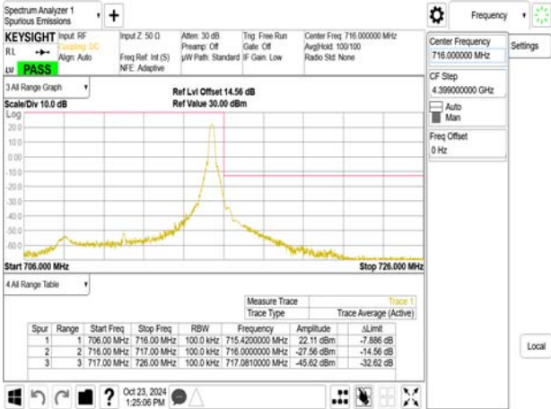
Band Edge_Band17_10MHz_OPSK_RB50_0_CH23780
