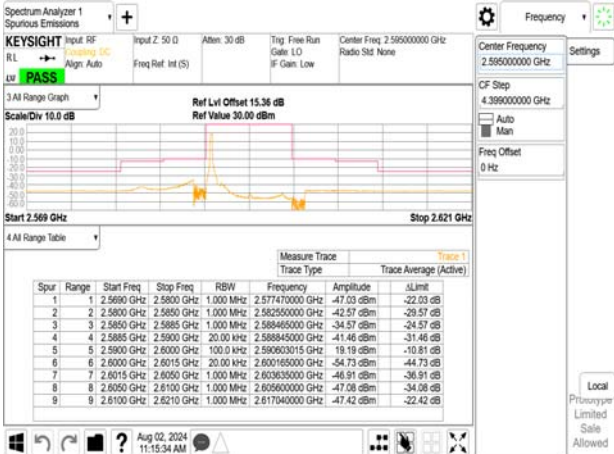
Emission Mask_Band38_10MHz_QPSK_RB1_0_CH38200
