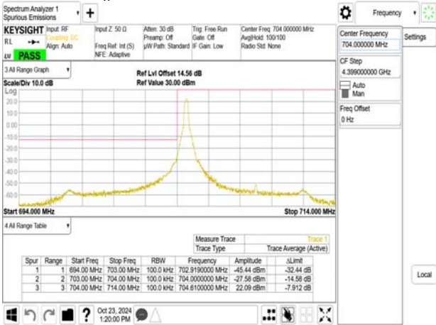
Band Edge_Band17_10MHz_OPSK_RB1_49_CH23800
