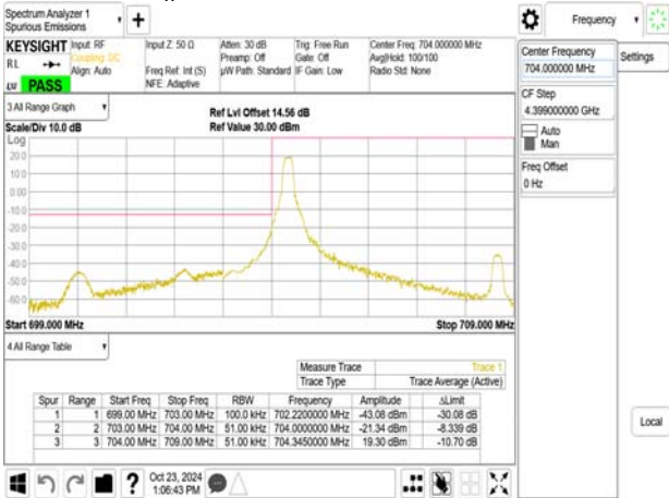
Band Edge_Band17_5MHz_OPSK_RB1_0_CH23755
