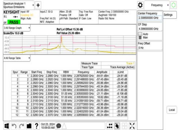
Emission Mask_Band30_5MHz_OPSK_RB1_0_CH27710
