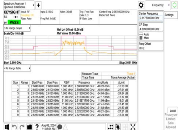
Emission Mask_Band38_5MHz_QPSK_RB25_0_CH38225
