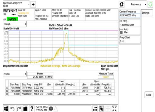
Emission Mask_Band26-Part90s_1.4MHz_QPSK_RB1_5_CH26783
