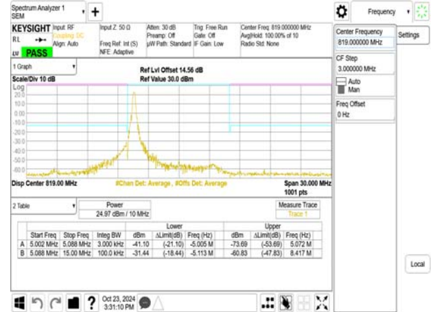
Emission Mask_Band26-Part90s_10MHz_QPSK_RB1_49_CH26740
