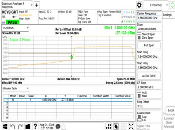
Band Edge_Band25_10MHz_OPSK_RB50_0_CH26640
