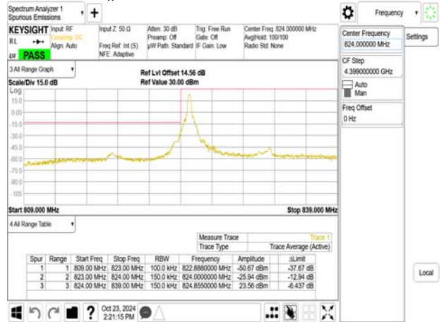
Band Edge_Band26_15MHz_QPSK_RB1_0_CH26865
