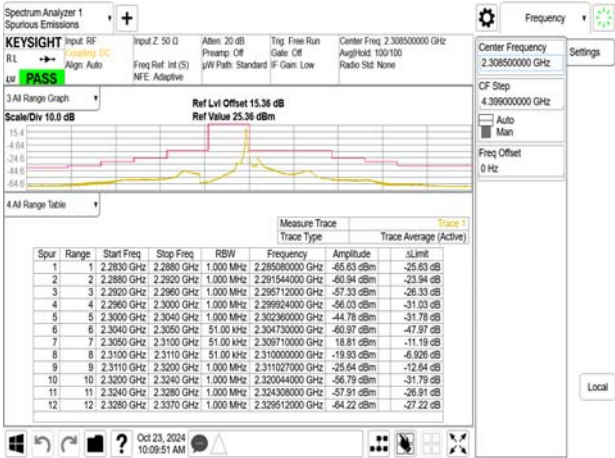
Emission Mask_Band30_5MHz_QPSK_RB1_24_CH27710
