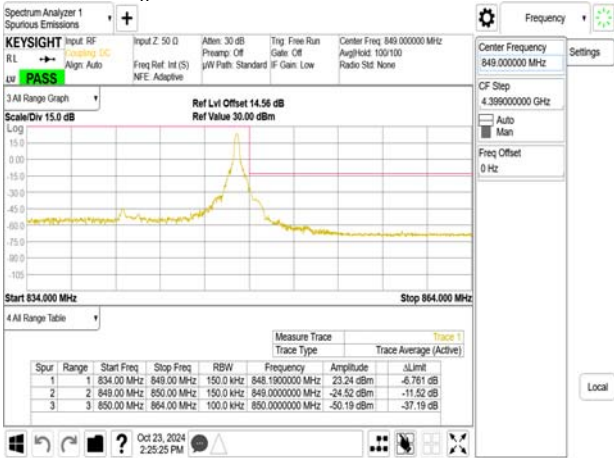
Band Edge_Band26_15MHz_OPSK_RB75_0_CH26865
