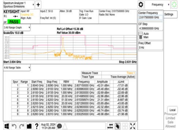
Emission Mask_Band38_5MHz_OPSK_RB1_0_CH38225
