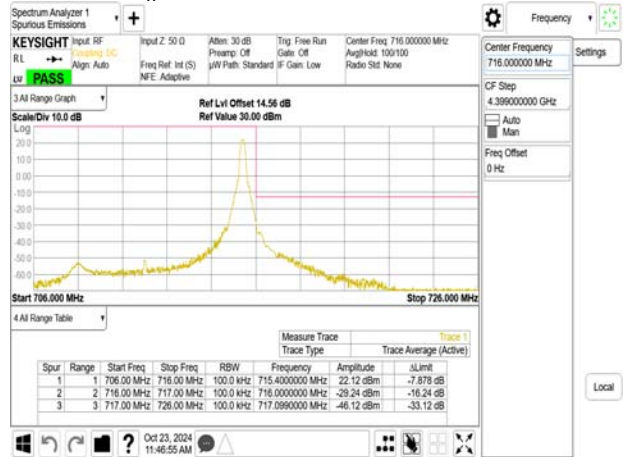
Band Edge_Band12_10MHz_OPSK_RB1_49_CH23130
