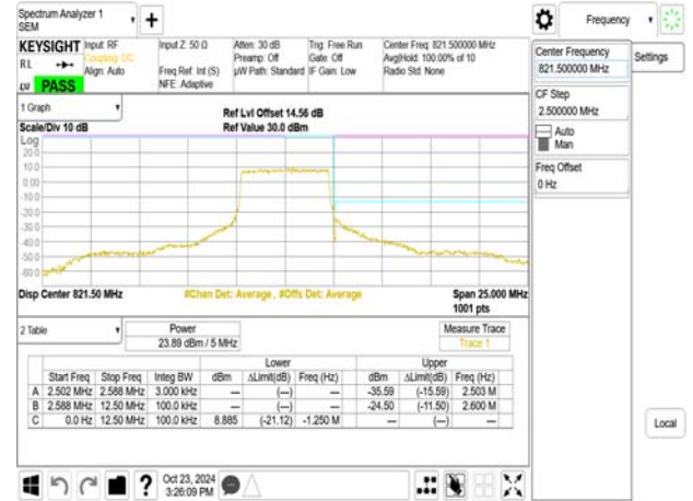
Emission Mask_Band26-Part90s_10MHz_QPSK_RB1_0_CH26740
