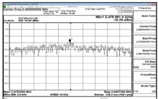
Power Density_BLE_2M_HighCH39-2480
