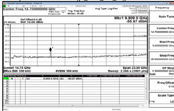
Spurious Emission High_BLE_1M_HighCH39-2480
