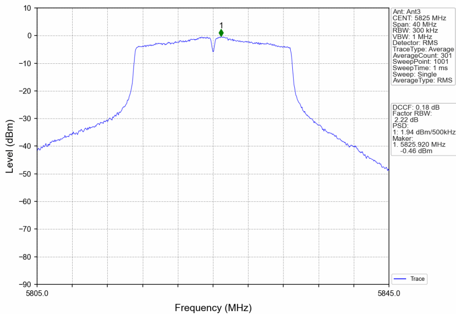
802.11n(HT20)_HCH_5825MHz_Ant3_NTNV
