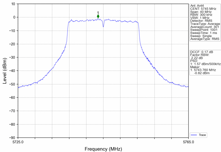
802.11a_LCH_5745MHz_Ant4_NTNV
