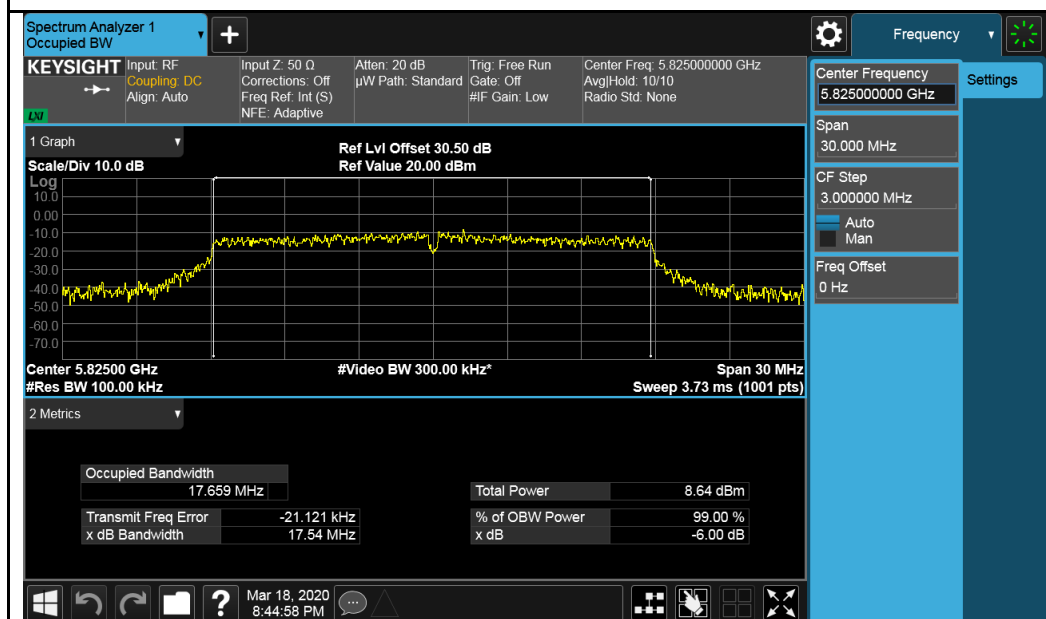
802.11n-HT20-5825MHz
