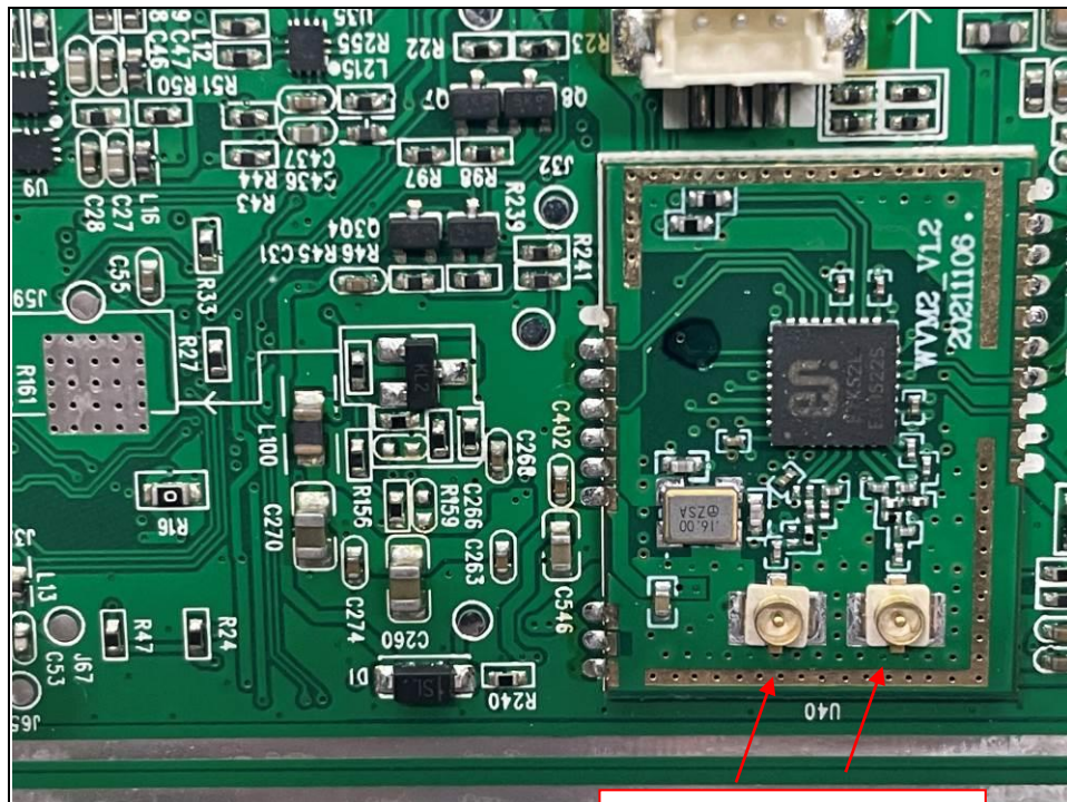
5.8GHz SRD Antenna TX/RX Connector
