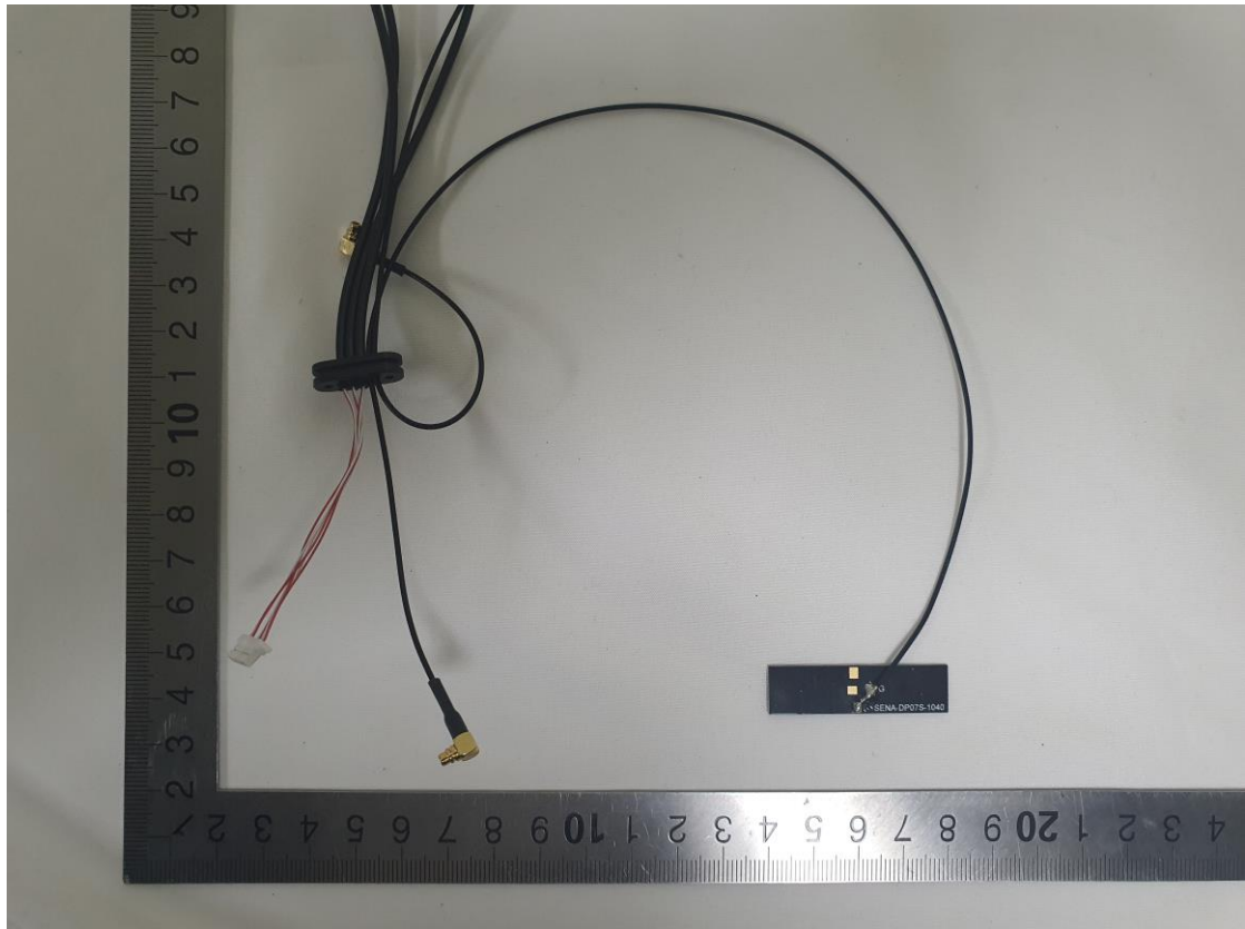
MESH Antenna 1
