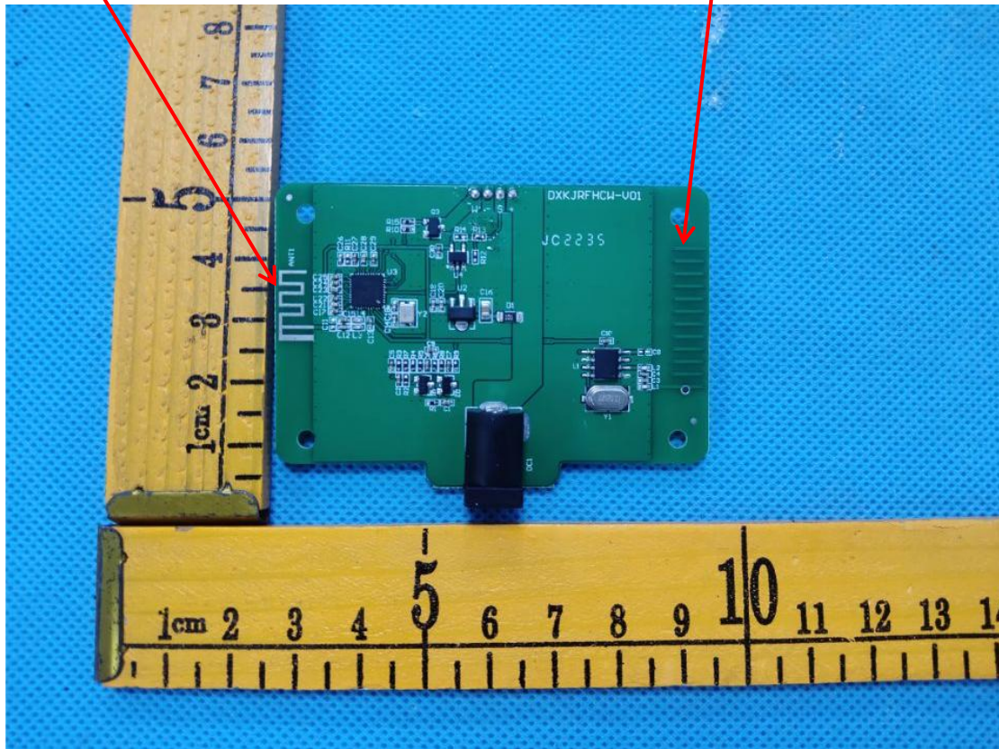
433MHz Antenna(Receiving)
