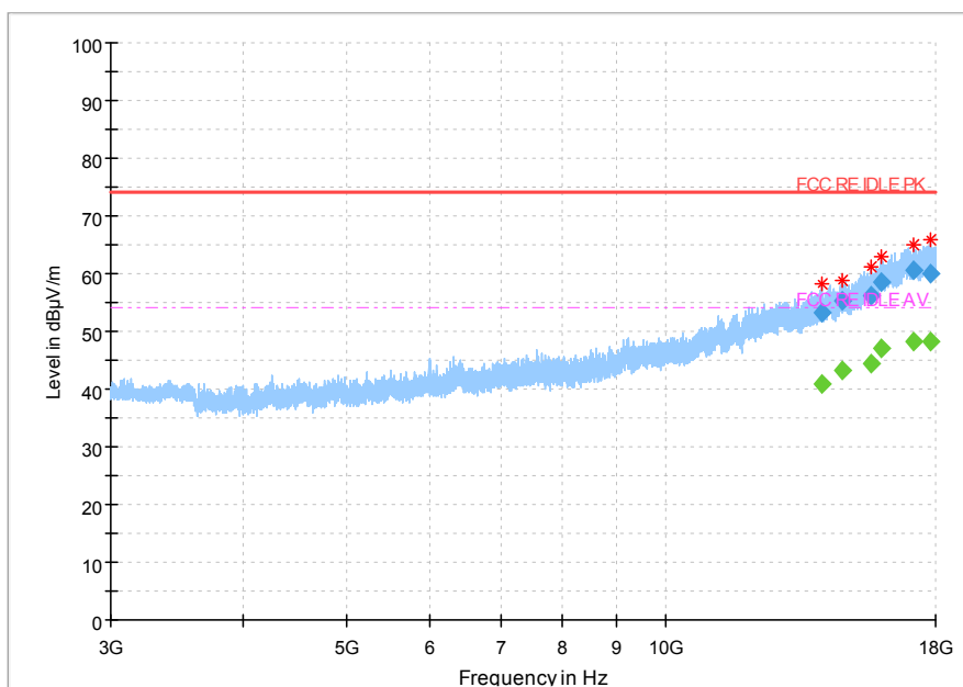
Fig.28 Radiated emission: CH39, 3GHz~18GHz
