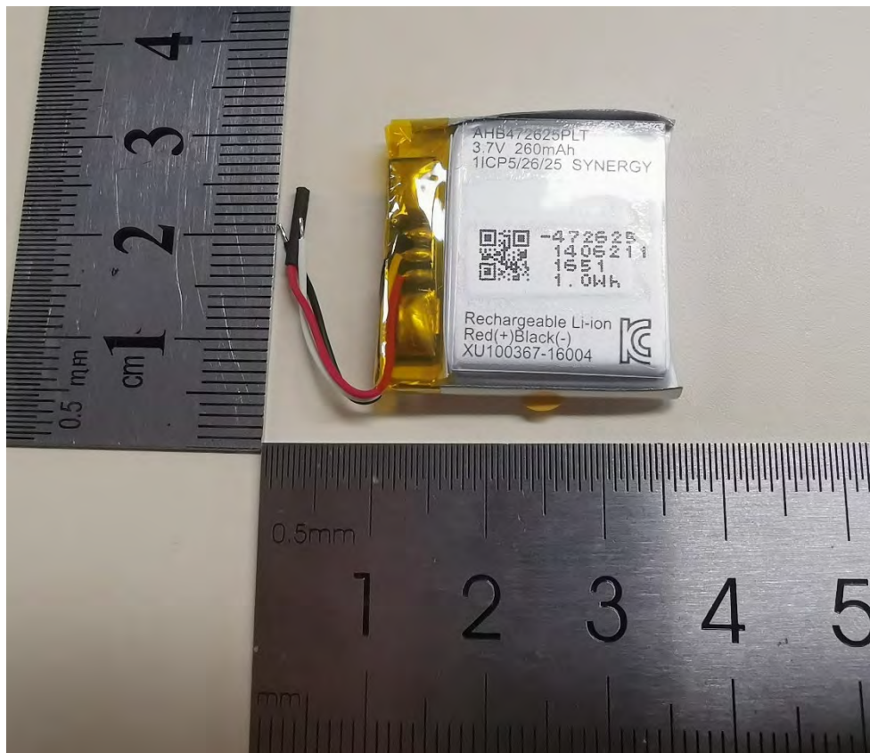
(42) EUT Photo
