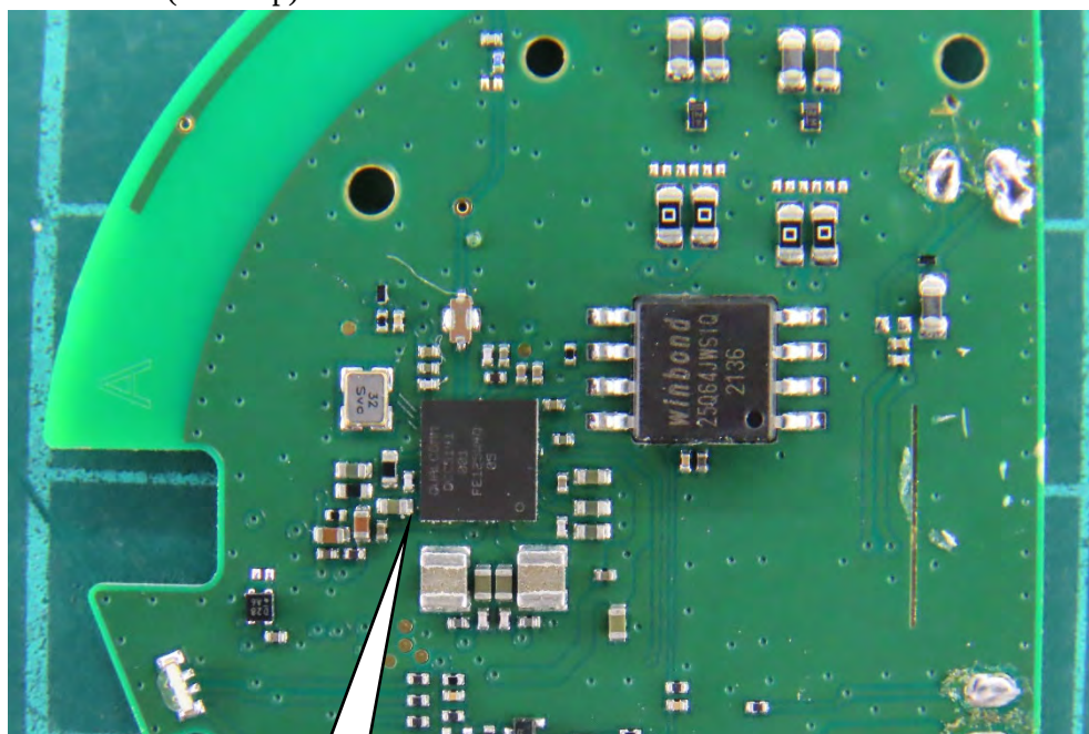
(29) EUT Photo(RF Chip)
