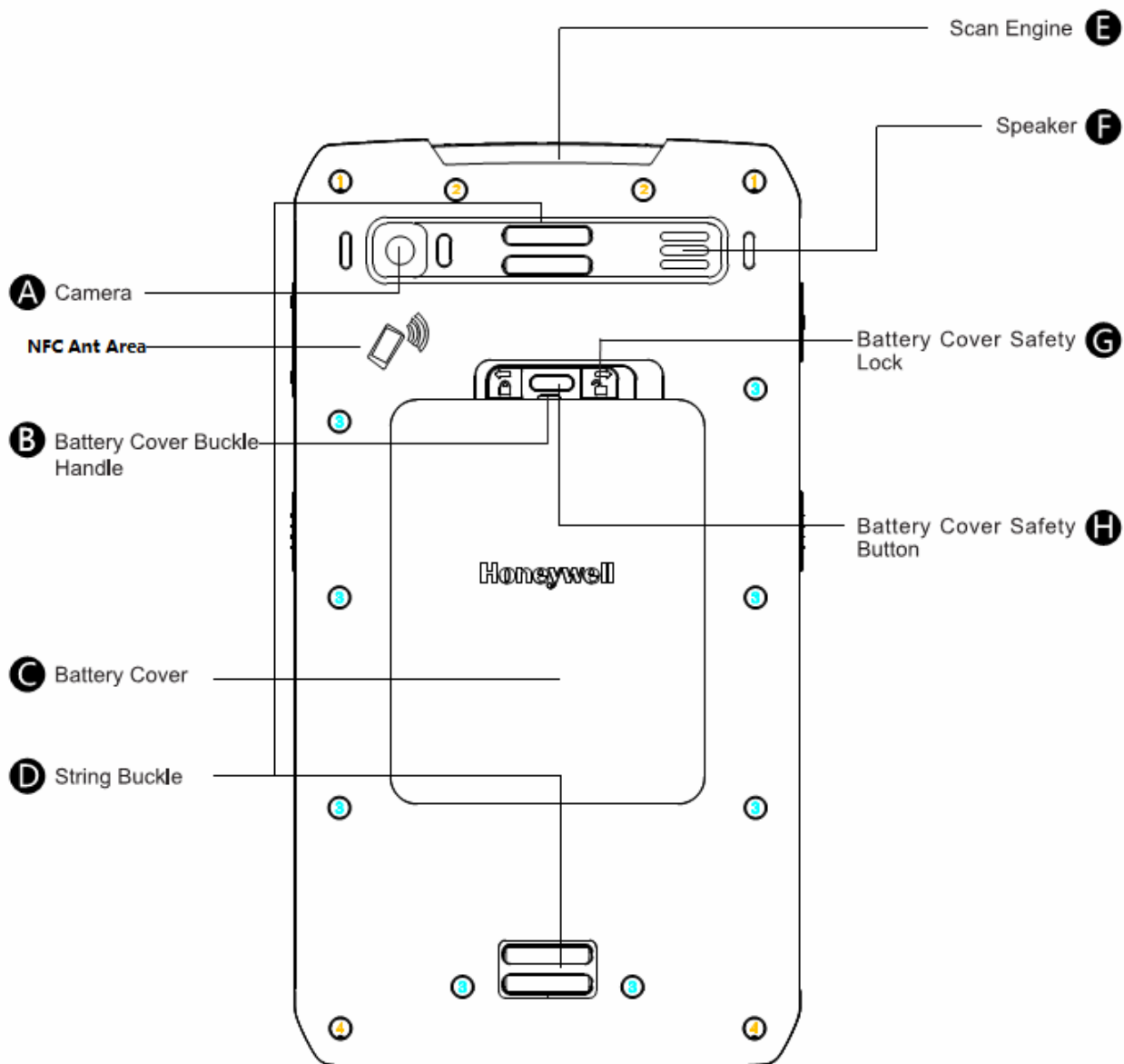
Back view of the EDA70-3
