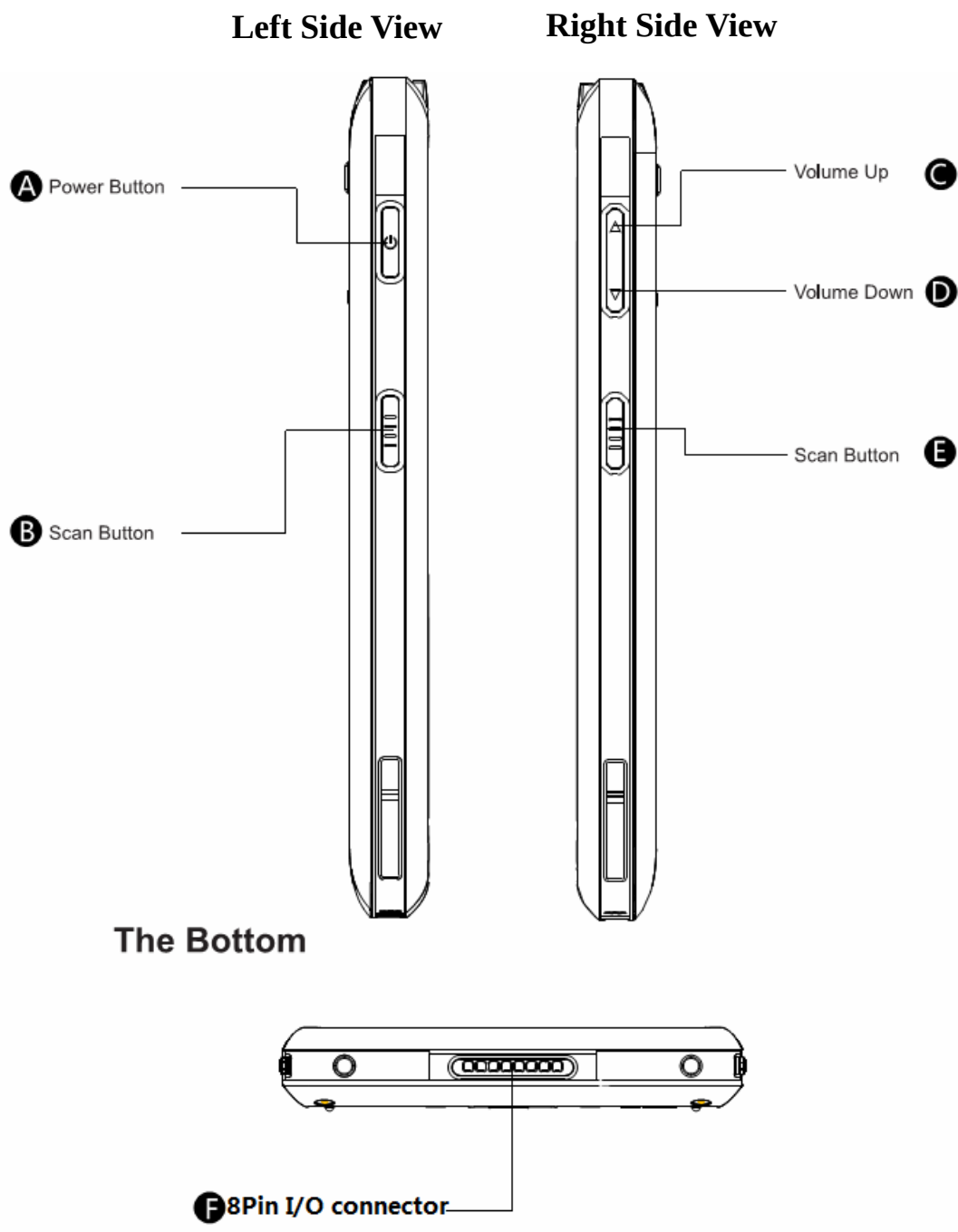
Side and bottom views of the EDA70-3
