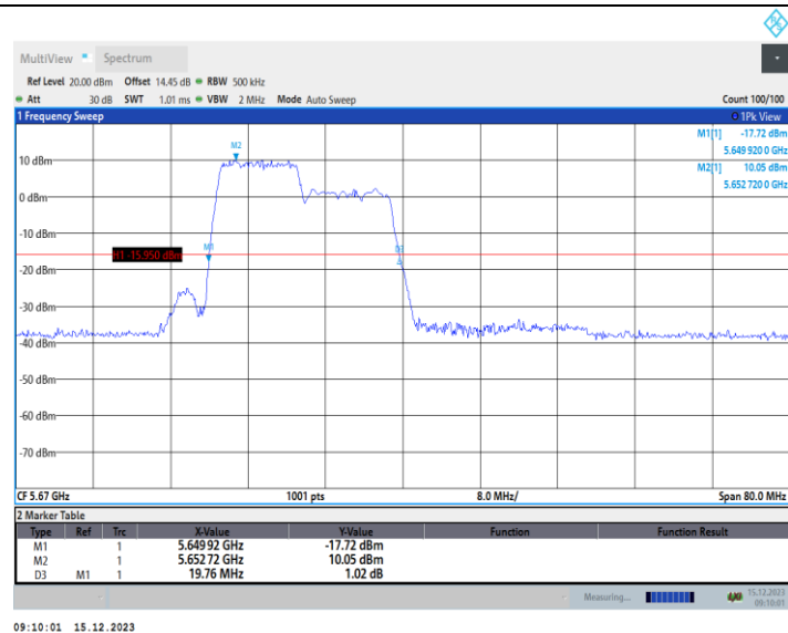
11AX40MIMO Ant1_5670_242Tone_RU61
