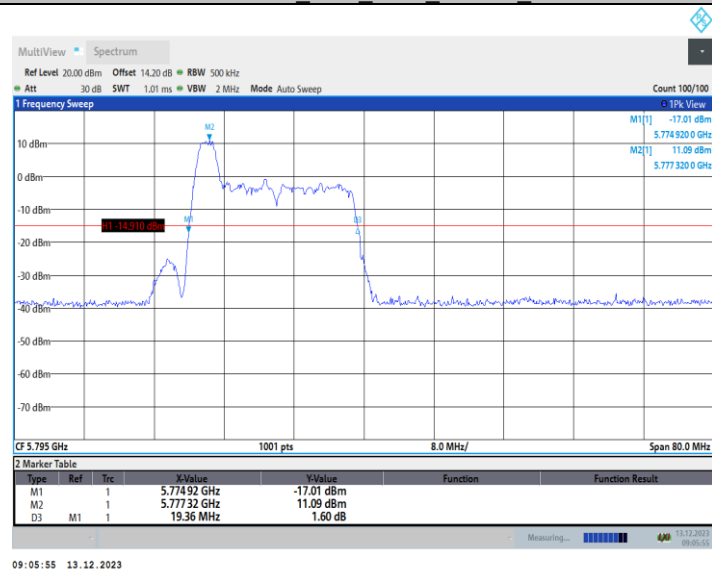
11AX40MIMO Ant1_5795_52Tone_RU37
