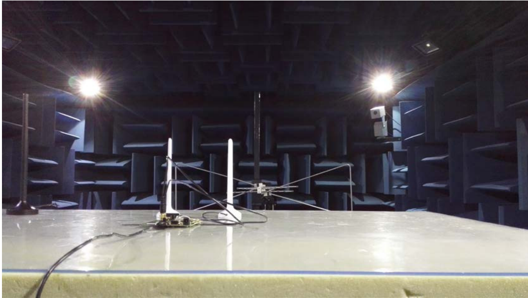
Radiated Spurious Emission (below 3GHz)
