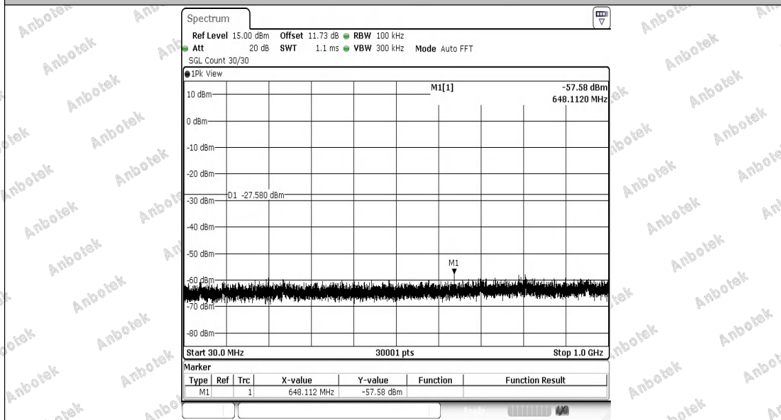
3DH5-Ant1-2480-30~1000-PASS
