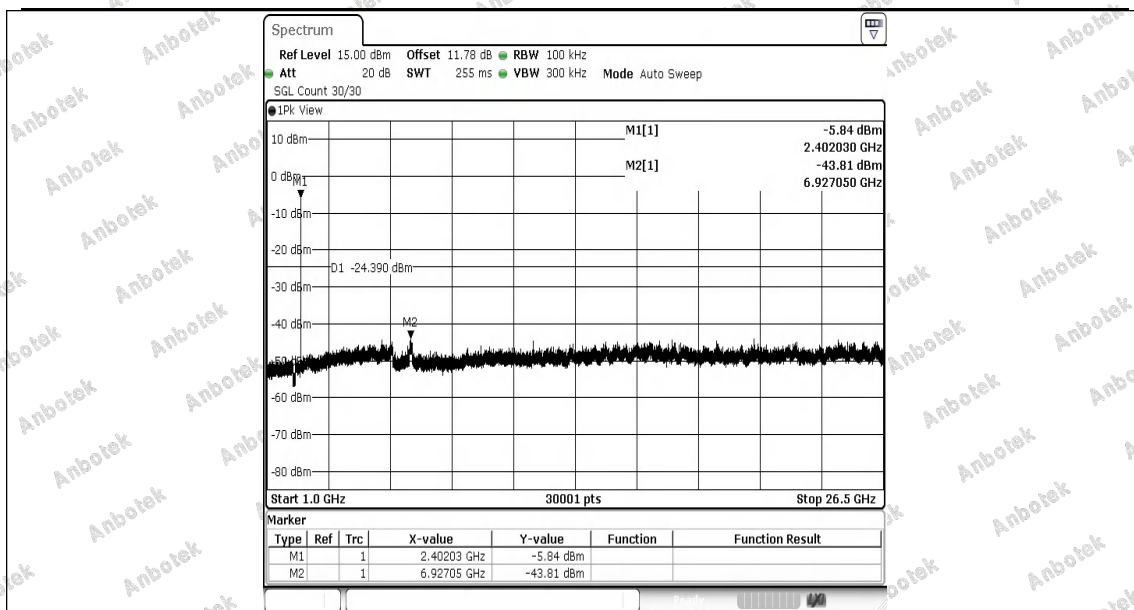
3DH5-Ant1-2402-1000~26500-PASS
