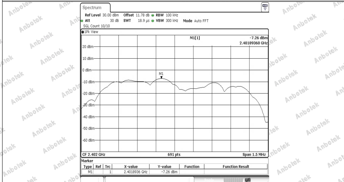
2DH5-Ant1-2402-0~Reference-PASS
