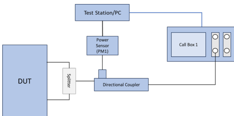
(b) Appendix B – Test Setup Photo 5
